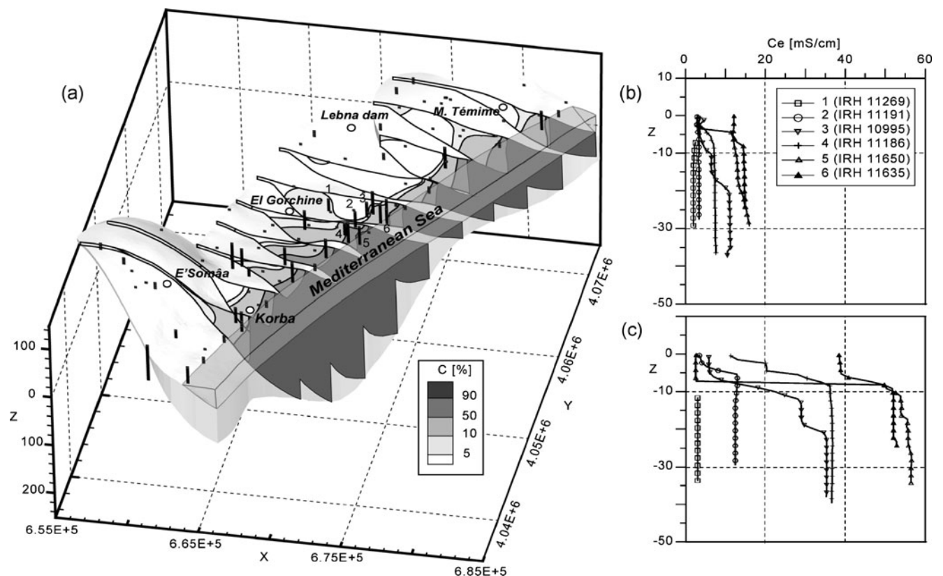
Fig. 3 Salinity description: a three-dimensional kriging of 854 data points; August 2004 vertical logs and surface measurements are represented by black squares or black bars; b vertical salinity logs of December 1996; c vertical salinity logs of August 2004. Z stands for elevation
