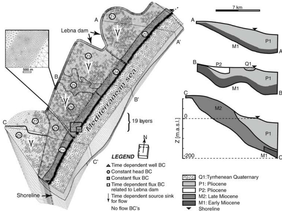
Fig. 9 The Korba aquifer 3D numerical model and three flow material cross-sections ( W zoom window). Note that wells are attributed to the third slice and lateral fluxes are integrated on the thickness of the Pliocene only. The zonation (Z1–Z10) used for inverse calibration is also shown
