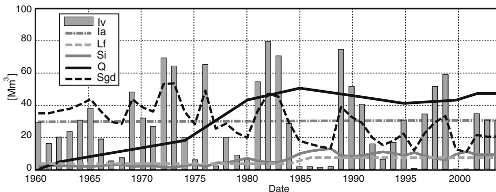
Fig. 13 Time evolution (1960–2004) of water budget in the Korba aquifer: Iv time dependent recharge, Ia average annual recharge, Lf lateral recharge with recharge from Lebna dam starting from 1986, Si seawater fluxes entering the system, Q pumping, Sgd submarine groundwater discharge
