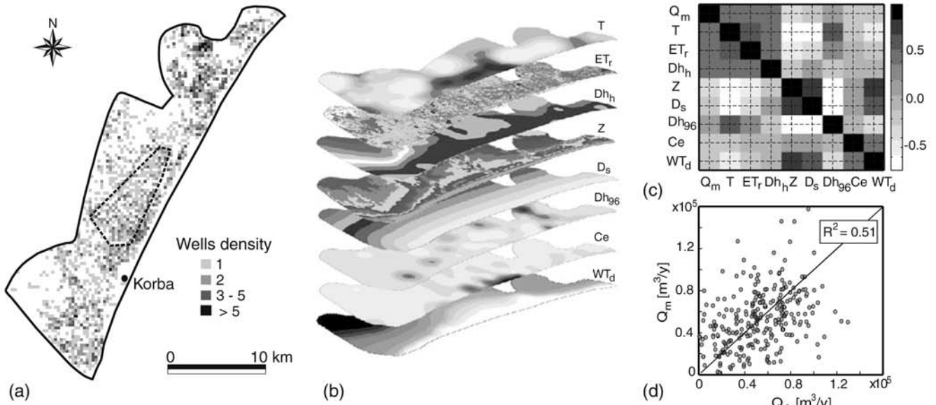
Fig. 7 a Wells density and area of the exhaustive pumping rate survey ( dashed line polygon ). Wells are grouped into 1,491 clusters on a regular grid of 300 \times 300 m cell size. b Eight maps with the secondary information. The eight parameters are: aquifer transmissivity ( T ), summer 2000 crop evapotranspiration ( ET_r ), December 1996 electrical conductivity ( Ce ), 1996 seasonal head variation ( Dh_{96} ), average 1996 water-table depth ( WT_d ), 1960–2004 historical piezometric decline ( Dh_h ), distance to the sea ( D_s ), and digital elevation model ( Z ). c Correlation matrix. d Scatter plot of estimated ( Q_c ) vs. measured ( Q_m ) pumping rates
