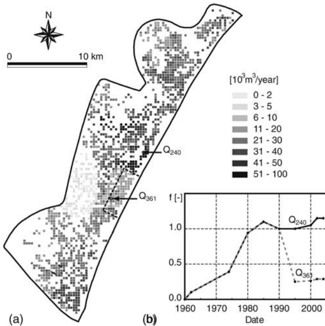
Fig. 10 a Average pumping rates ( Q 1996) with the area (delineated with dashed line ) where pumping was reduced in the 1990s. b Time-dependent evolution functions f [-] for both wells (solid black line for Q_{240} and gray dashed line for Q_{361} ) with 1996 extracted volumes as reference
