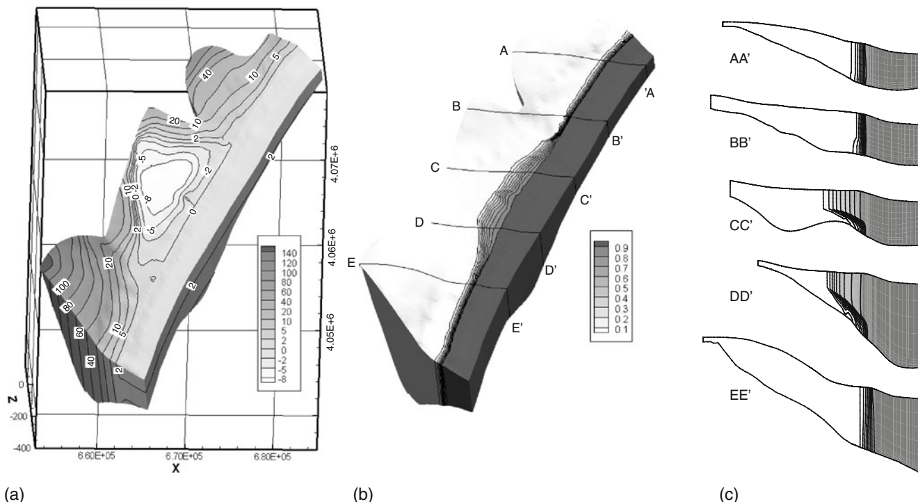
Fig. 12 a Three-dimensional views of simulated water-table elevation [m.a.s.l.] with non-standard contour intervals; b relative salt concentration [-] distribution; c cross-sections
