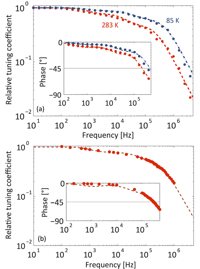
FIG. 1. Relative frequency-modulation of (a) QCL1 (at 85 K and 283 K) and (b) QCL2 (at 283 K) under direct current modulation ( I_{pp} = 0.2\text{ mA} ) and fitted model (dashed lines). The phase shift between frequency- and current-modulation is shown in the inset. In each case, the responses cannot be fitted with a one-pole low-pass filter but show a non-negligible roll-off and a significant phase shift above a few hundred hertz already. Then, a clear -20\text{ dB/decade} roll-off is observed above \sim 200\text{ kHz} . The modulation bandwidth of QCL1 increases when the device is operated at 85 K. At room temperature, QCL2 shows a higher frequency-modulation bandwidth than QCL1.
