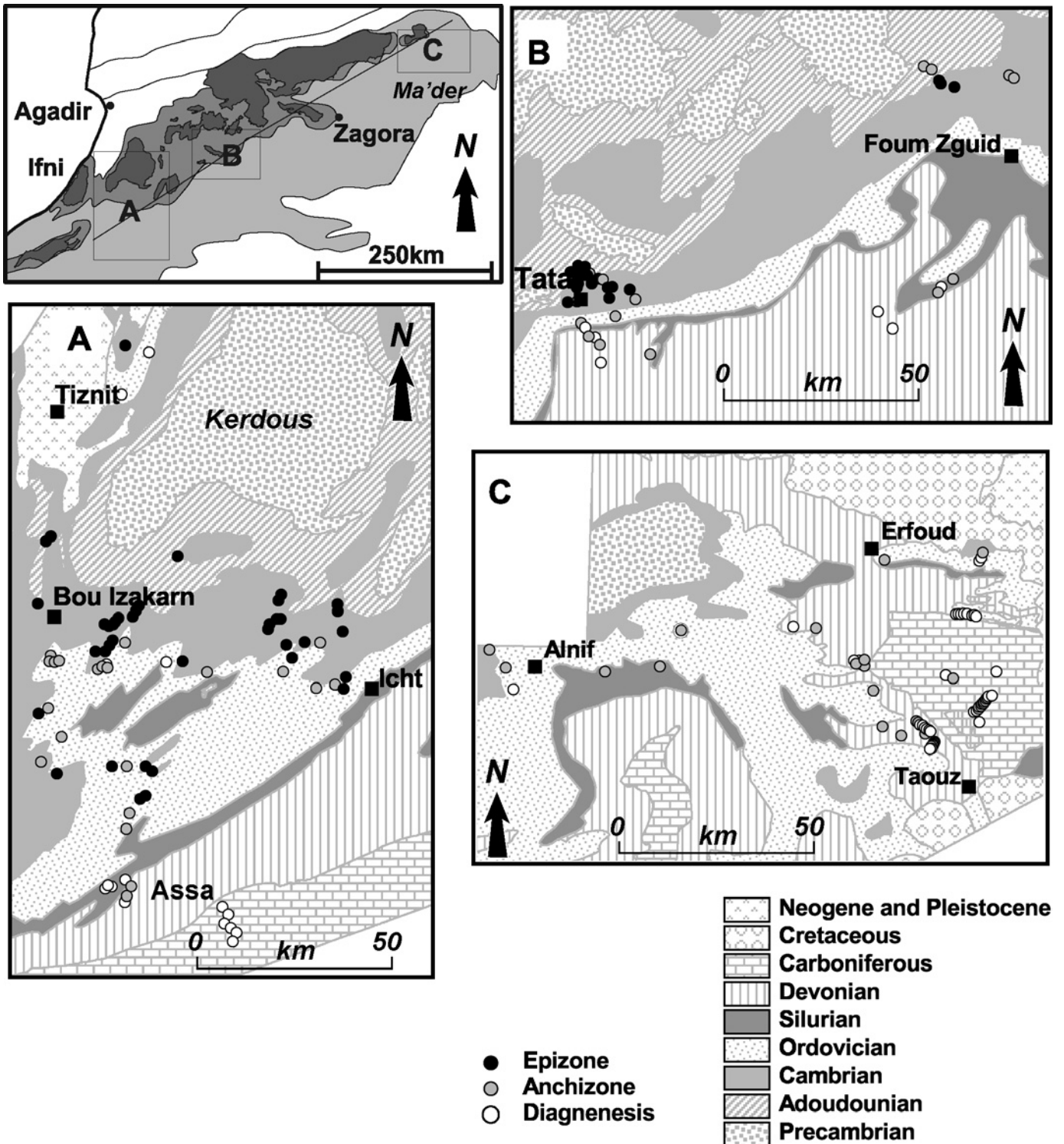
Fig. 2. Sampling map and results. Illite cristallinities from air dried samples ( <2 \mu ) for the three key areas on the southern flank of the Anti-Atlas. The Illite cristallinities outline low-grade metamorphic zones. In the southwestern and central Anti-Atlas all three low-grade metamorphic zones can be found. In these areas the correlation between IC and stratigraphy is fairly distinct. In the eastern Anti-Atlas epizonal samples are absent and no clear trend is recognizable.
