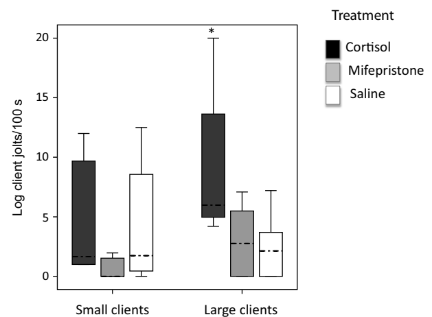
Fig. 2. The effect of glucocorticoids on the dishonesty level (jolts) of cleaner fish Labroides dimidiatus , measured in the field and compared with a control (saline), using the frequency of jolts per 100 s of inspection for clients of two different size categories. See Fig. 1 for boxplot definitions. Symbols above bars and sample sizes per treatment were the same as in Fig. 1.
