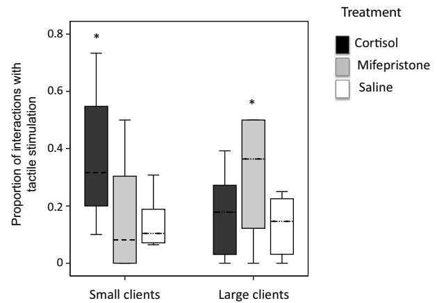
Fig. 1. The effect of glucocorticoids on the proportion of tactile stimulation provided by cleaner fish Labroides dimidiatus to client fish, compared with a control (saline) for clients of two different size categories. Medians (dashed lines) and interquartile range are presented in boxes. * above bars represent significant P values which refer to Mann-Whitney U tests for each glucocorticoid treatment against the reference (saline) group (*, <0.025 ). Sample sizes (number of individual cleaner fish) are n = 8 for all groups of treatments.
