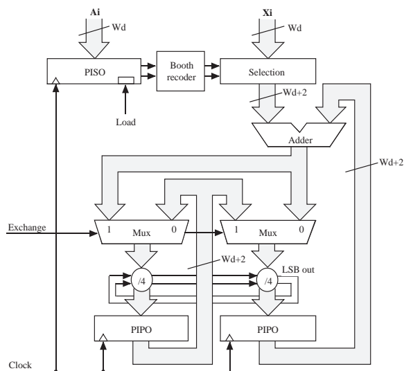
Figure 3: IMT-lp architecture: the scalar product processor
