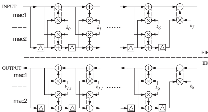
Fig. 5: data flow diagram of lattice FIR-IIR filter
