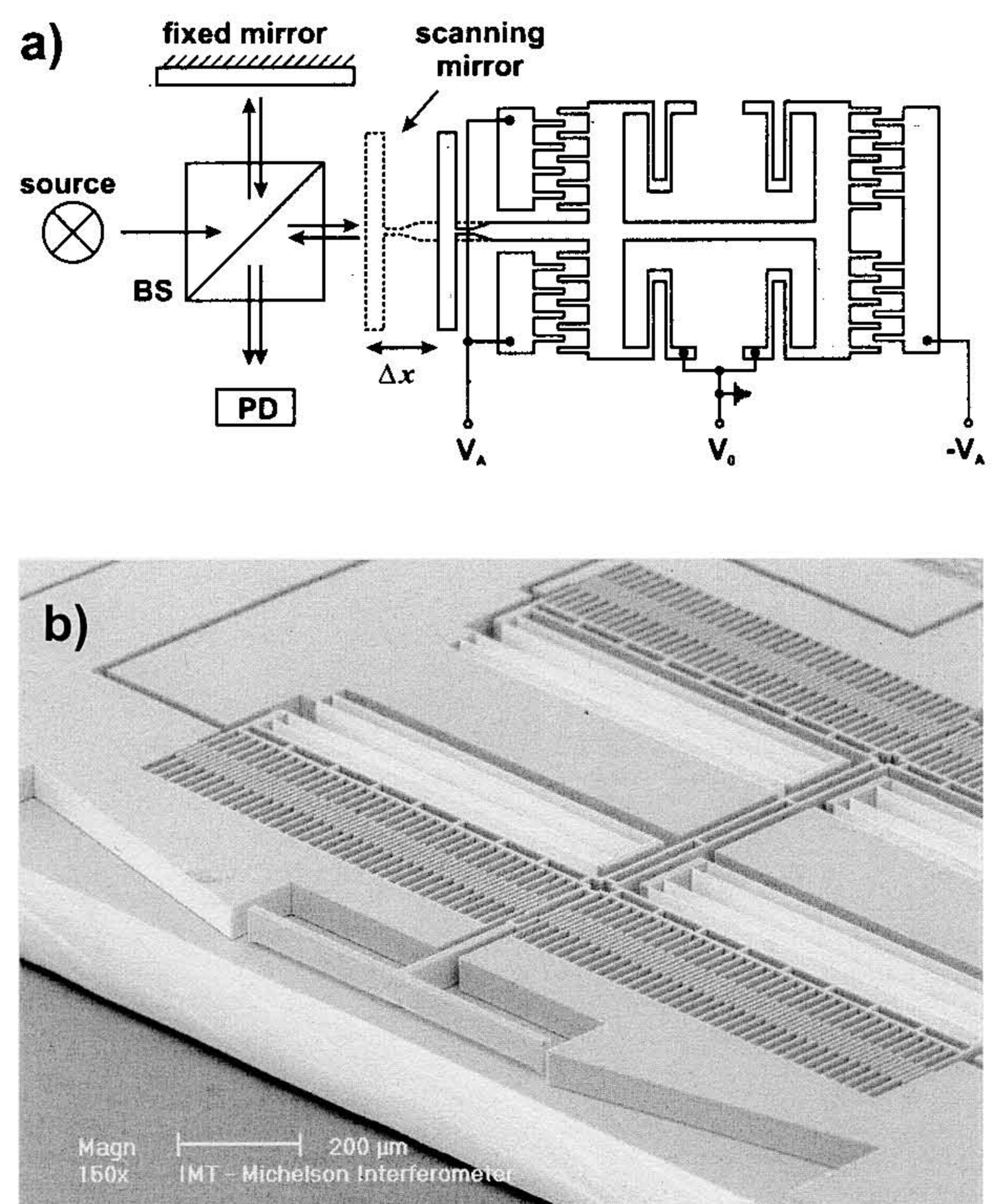
Fig. 5. a) Concept of Fourier transform spectrometer (FTS). In the real setup, the beam splitter (bs) and the fixed mirror are macroscopic. The movable mirror was driven by a push-pull configuration. b) The MEMS mirror is much larger than in the OXC and the VOA to increase the reflecting area.
