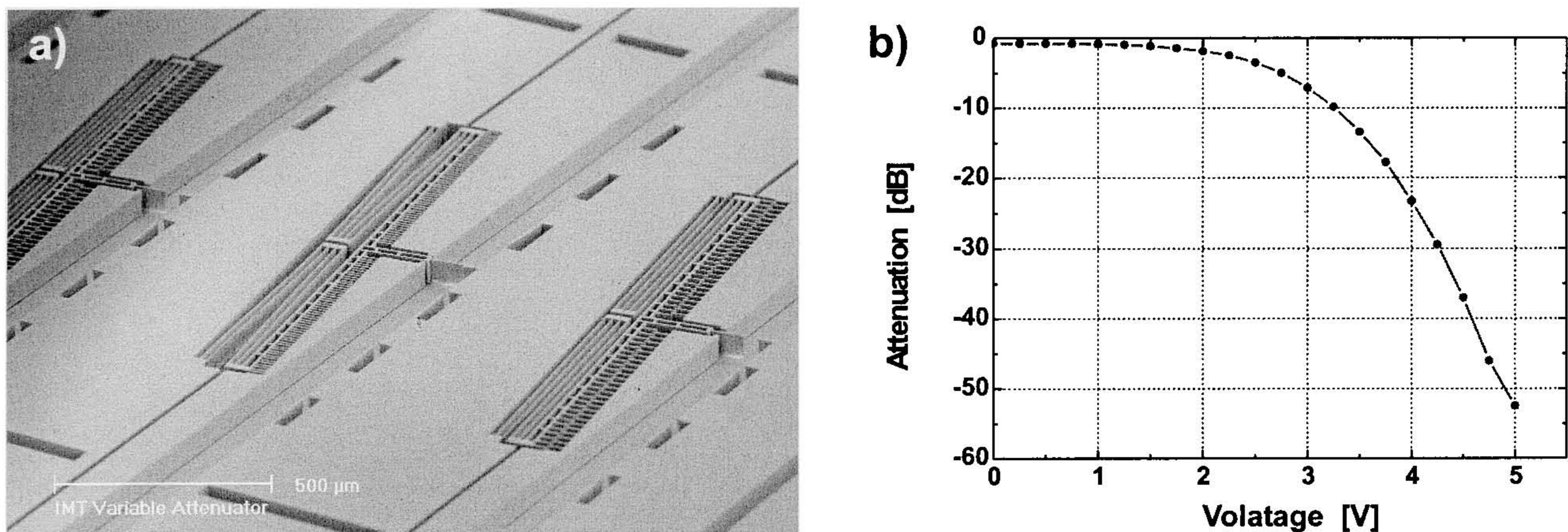
Fig. 4. a) The variable optical attenuator (VOA) moves a shutter in between two fibers. B) The attenuation of the VOA has a dynamic range of over 50 dB.
