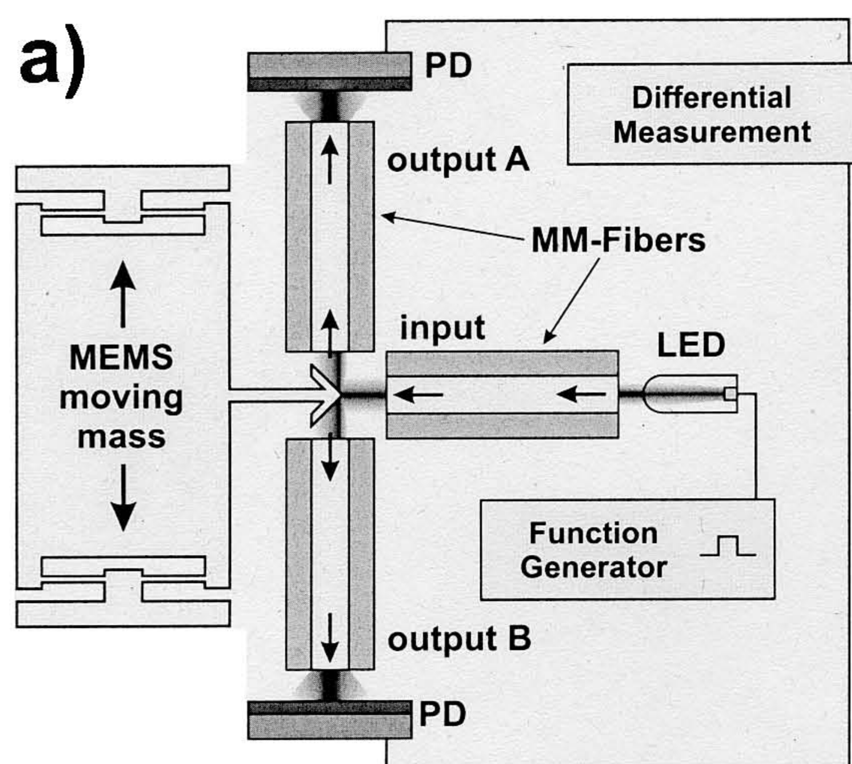
Fig. 6. a) In the optical MEMS accelerometer the light from the input fiber is split by a V-shaped mirror simultaneously into the two output fibers A and B. The signal from the photodetectors are subtracted from each other to achieve a differential measurement. The dynamic range of the usable and linear response of the moving mass is about 40 dB for \pm 6g at a bandwidth of 300 Hz. b) The fibers are inserted into the MEMS component via U-grooves and held by small leaf springs. The accelerometer is damped by a squeezed air film which is in a small gap in between the moving mass and the surrounding structure, which is visible in the upper left corner.
