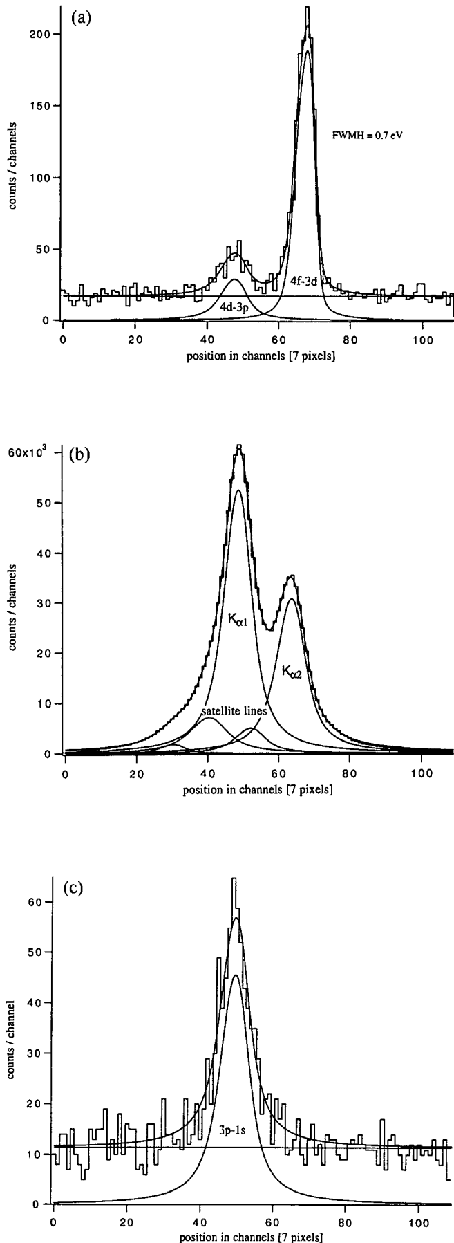
FIG. 2. (a) Position spectrum of 4F-3D and 4D-3P pionic beryllium lines. As the 4F-3D natural line width is very small, this spectrum was used to determine the energy resolution of our crystal spectrometer. (b) Argon K\alpha x-ray position spectrum used for calibration. The two lines, K\alpha_1 and K\alpha_2 , are separated by 2.13 eV. On the x axis, one channel corresponds to seven pixels = 157.5 \mu\text{m} . The fit function is a sum of six Voigt profiles ( K\alpha_1 , K\alpha_2 , and satellite lines) with the resolution function obtained from the 4F-3D pionic Be line (a) folded in. The positions and intensities of the satellite lines were taken from the NIST spectrum. (c) Pionic deuterium 3P-1S x-ray position spectrum. After taking into account the spectrometer movements, the comparison of the peak position with the argon K\alpha_1 peak position of (b) yields the transition energy. The total decay width \Gamma_{1S} is obtained after deconvoluting the instrumental resolution function of (a).
