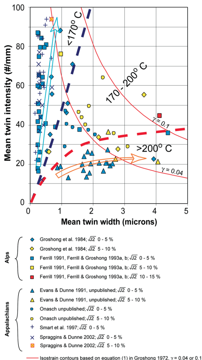
Fig. 3. Graph of mean twin intensity versus mean twin width with data points colored according to twin strain. Orange and blue arrows illustrate paths of increasing strain for temperatures > 200 and < 170 °C, respectively. Red lines are isostrain contours derived from Eq. (1) in Groshong (1972).
