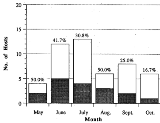
Fig. 3. Seasonal distribution of Turdidae parasitized by infected Ixodes ricinus ticks.
