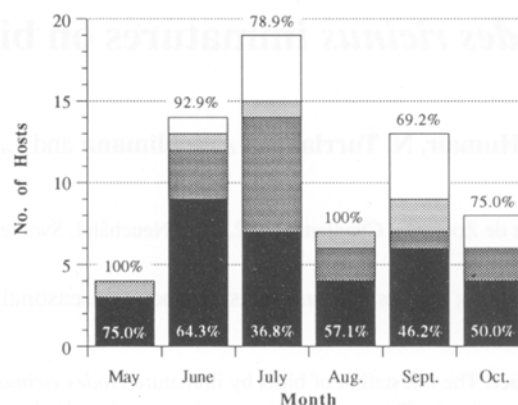
Fig. 1. Seasonal distribution of Turdidae infested with Ixodes ricinus immatures, Staatswald, Switzerland, May – October 1988.
