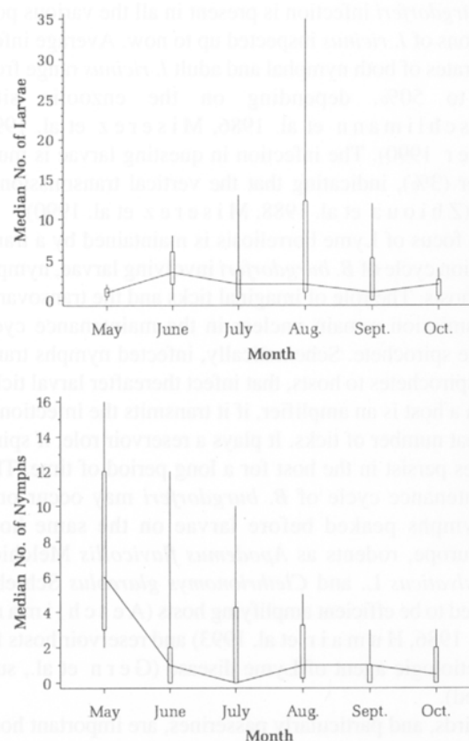
Fig. 2. Seasonal distribution of the median number of Ixodes ricinus larvae (2a, above) and nymphs (2b, below) per Turdidae. — median number of tick per host □ delimits the percentiles 25 and 75 | delimits minimal and maximal values
