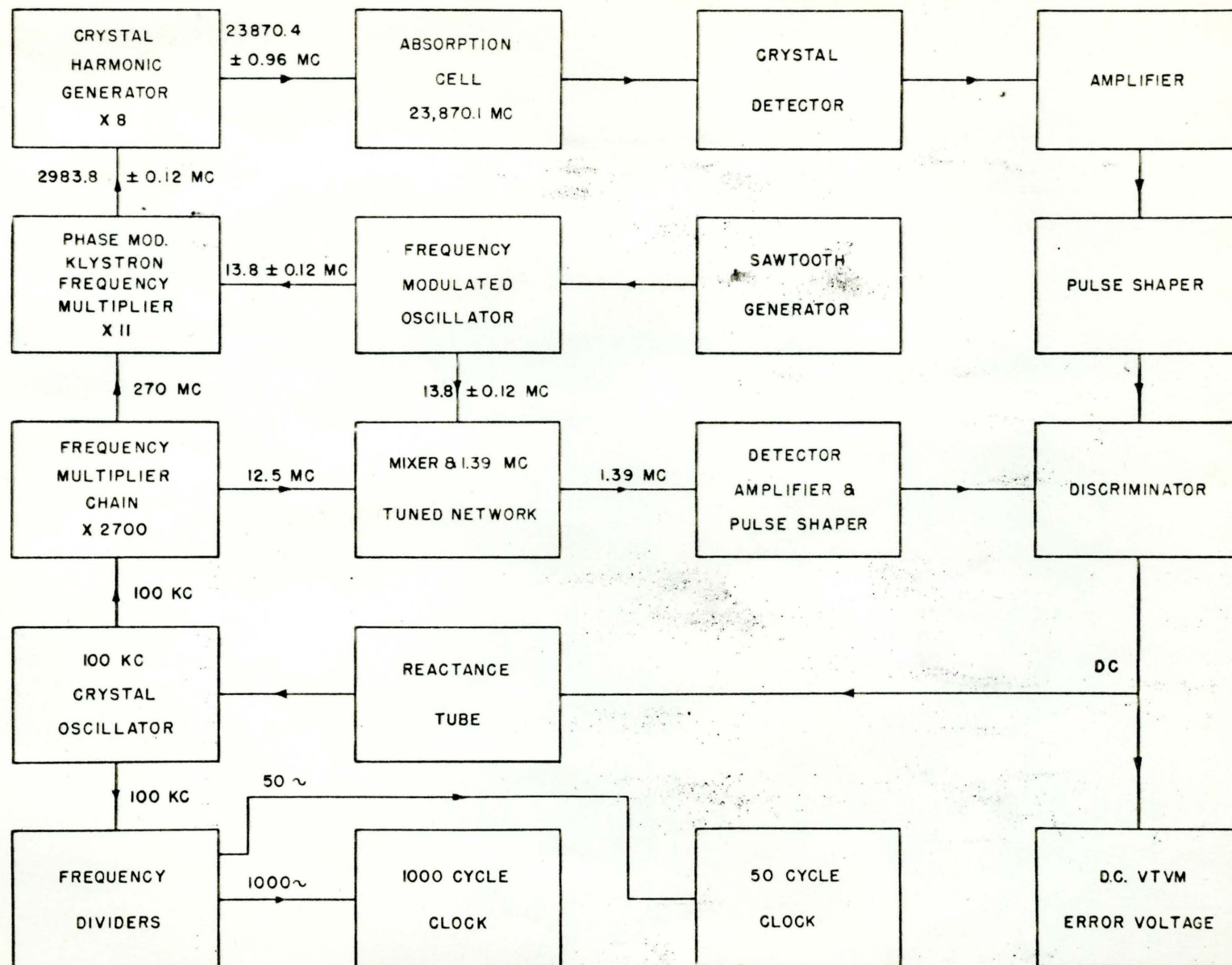
COMPLETE BLOCK DIAGRAM OF NBS ATOMIC CLOCK FIGURE 7
