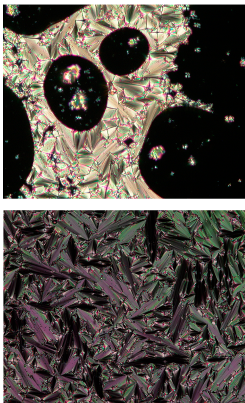
Figure 3. Thermal-polarized optical micrographs of the focal-conic fan textures of the SmA-like phase displayed by P_2 , at T = 150 °C (top) and P_3 , at T = 145 °C (bottom) upon cooling the samples from the isotropic liquid.
