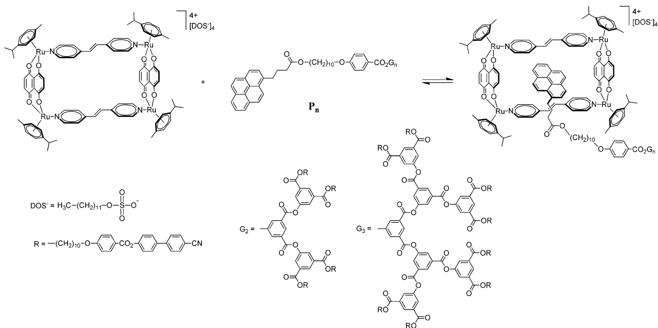
Scheme 2. Synthesis of the [P_n \subset 1][DOS]_4 Assemblies a
