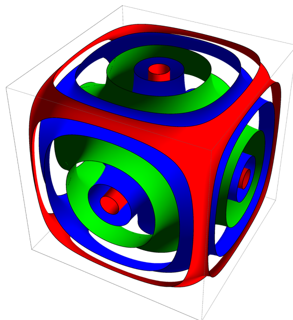
Figure 9. Schematic representation of the multicontinuous cubic structure (surface foliation model 34,37,38 ) for the host-guest complex [P_2 \subset I][DOS]_4 : Representation of the different intermediate interfaces \beta (red for the aliphatic/dendritic interfaces, |\beta| = 1.89 ; blue for the mesogen/aliphatic interfaces, |\beta| = 1.44 ) on both sides of the isosurface of zero-mean curvature ( \beta = 0 , green).
