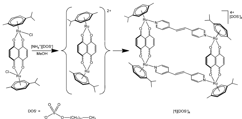
Scheme 1. Synthesis of the Arene Ruthenium Metallacycle Isolated As Its Dodecyl Sulfate Salt, [1][DOS]_4 a
