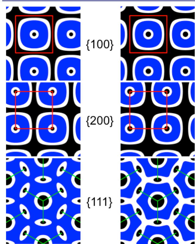
Figure 10. Simulated distribution of segregated zones in the cubic cell for complexes [P_2 C 1][DOS]_4 (left), and [P_3 C 1][DOS]_4 (right), within most important crystallographic families of planes (blue: mesogens + metallacycles sublayers; white: aliphatic strata; black: dendritic cores labyrinths; red frame: cubic lattice; green lines: edges to vertices from next plane).
