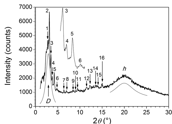
Figure 7. Representative SAXS patterns of [P_3 \subset 1][\text{DOS}]_4 at T = 80 \text{ }^\circ\text{C} .
