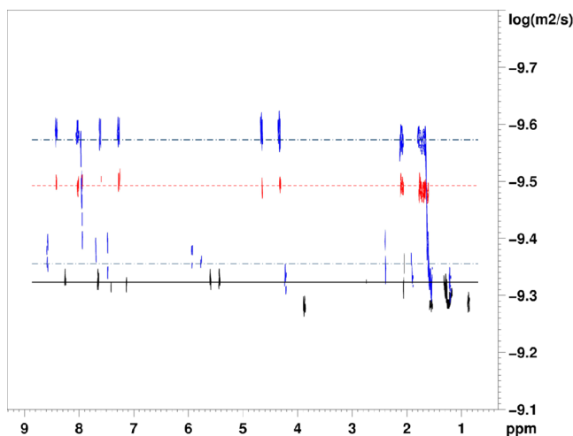
Figure 2. DOSY NMR spectra of P_3 (red), [1]^{4+} (black) and the corresponding associated system (blue) in CD_2Cl_2 at 21 °C.
