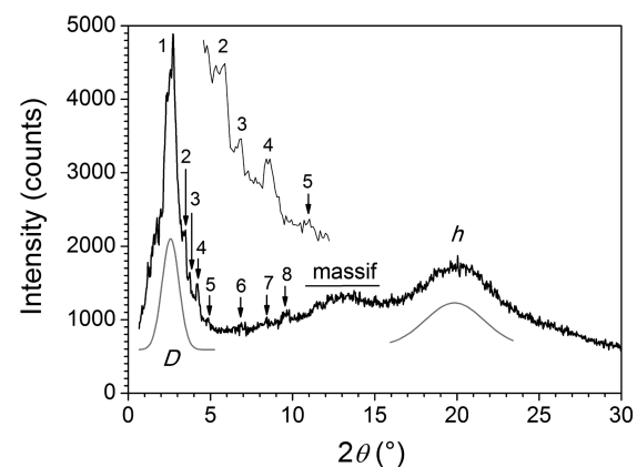
Figure 8. Representative SAXS patterns of [P_2 \subset 1][\text{DOS}]_4 at T = 80 \text{ }^\circ\text{C} .
