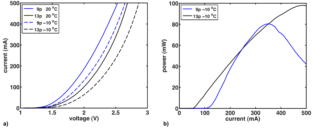
Fig. 2. (a) IV curves of the two different devices measured at -10\text{ }^{\circ}\text{C} (dashed) and 20\text{ }^{\circ}\text{C} (solid). (b) Multimode LI curves at -10\text{ }^{\circ}\text{C} measured in a simple straight cavity using an OC with a radius of curvature of 15 mm and a transmission depending on the field enhancement (9 pairs: 5.7%, 13 pairs: 10.6%)
