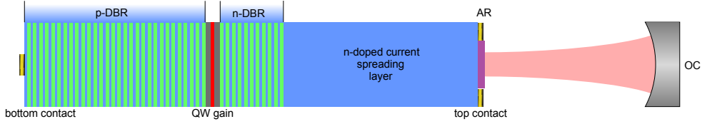
Fig. 1. Schematic of an electrically pumped (EP) VECSEL gain chip with the external cavity (not to scale): Bottom disc contact and top ring electrode inject current into the structure. The p-DBR acts as end mirror for the laser wavelength. The gain section consists of several quantum wells (QWs), the partial-reflective intermediate n-DBR increases the field enhancement. The current spreading layer (CSL) supports a homogeneous current injection to the center of the device. The dielectric anti-reflection (AR) coating reduces unwanted sub-cavity effects from the CSL. A curved output coupler (OC) completes the laser cavity.
