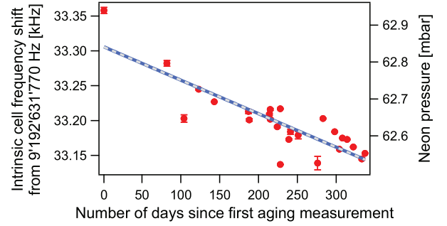
FIG. 3. Temporal evolution of the intrinsic cell frequency and buffer gas pressure as a function of time for cell sample 1. Red circles: experimental data. Solid blue line: exponential fit from Eq. (1). Dashed grey line: linear fit.
