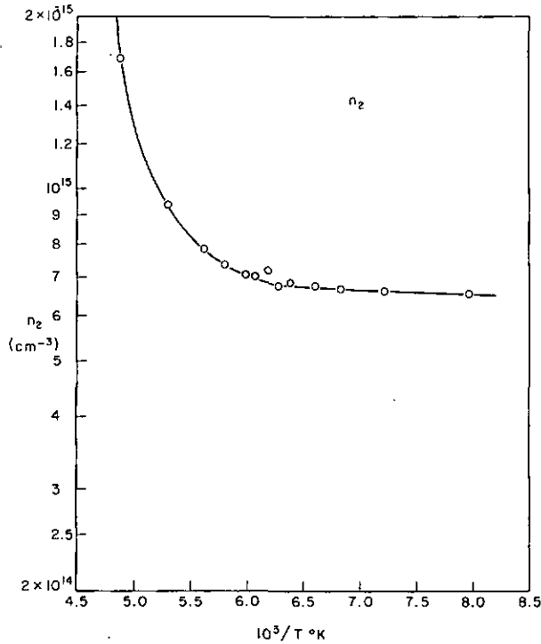
Fig. 8 Concentration of *slow* holes versus temperature
