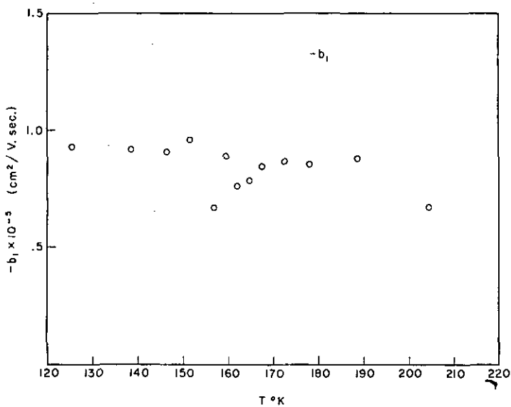
Fig. 10 Mobility of electrons versus temperature
