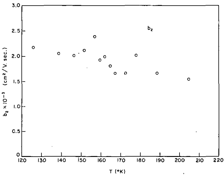
Fig. 11 Mobility of «slow» holes versus temperature
