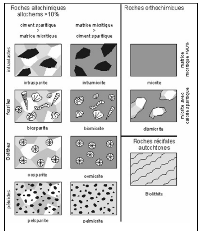
Fig 5.3 Classification de Folk (1962).
