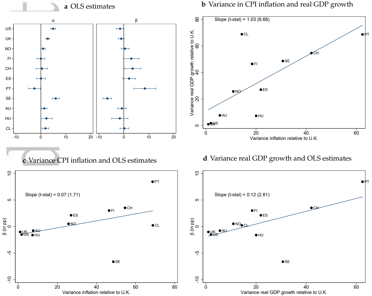
Figure 3: Volatility of historical data and OLS estimates
