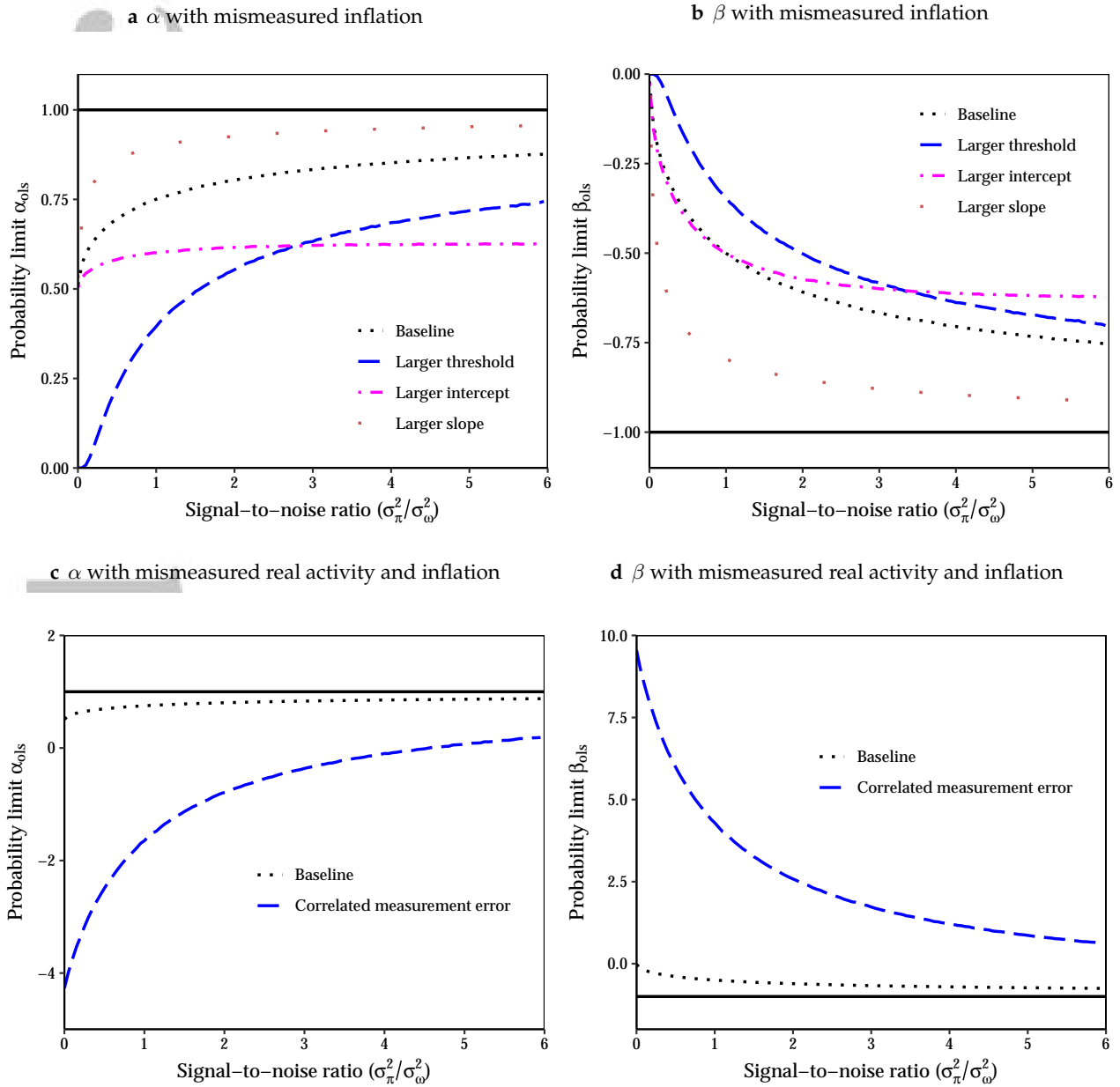
Figure 1: Simulated probability limit
