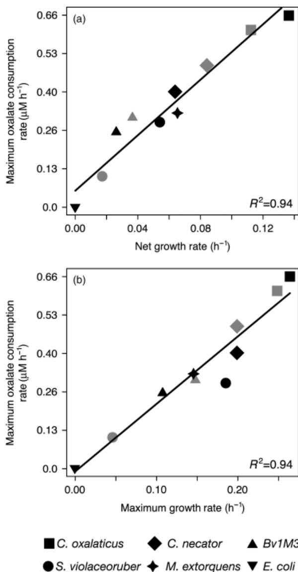
Fig. 3. Data showing the correlation between the net growth rate ( \mu ) (a), maximum growth rate ( \mu_{\text{max}} ) (b), and the maximum oxalate consumption rate for the six strains tested. The black symbols are for data obtained using potassium oxalate and the gray symbols are for data obtained using calcium oxalate. The correlation coefficient is indicated at the bottom of each panel.
