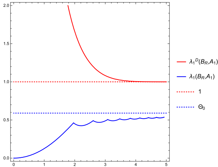
Fig. 1. First magnetic Dirichlet eigenvalue (in red) of a disk B_R as a function of R ; first magnetic Neumann eigenvalue (in blue) of a disk B_R as a function of R . Here \beta = 1 . (For interpretation of the colors in the figure(s), the reader is referred to the web version of this article.)
