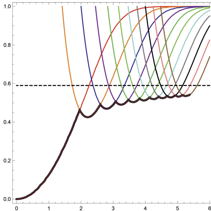
Fig. 3. Analytic branches \lambda_1(n, 1, R) , n = 0, \dots, 10 . In particular n = 0 (red), n = 1 (orange), n = 2 (blue), n = 3 (purple), n = 4 (dark green), n = 5 (light green), n = 6 (cyan), n = 7 (gray), n = 8 (black), n = 9 (pink), n = 10 (brown). Here the variable on the abscissae axis is the radius R . The first eigenvalue is given by the minimum of all analytic branches, and is highlighted in dark brown. (For interpretation of the colors in the figure(s), the reader is referred to the web version of this article.)
