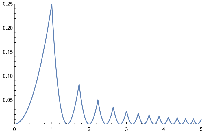
Fig. 2. First eigenvalue on a circle of radius R as a function of R , for \beta = 1 .
