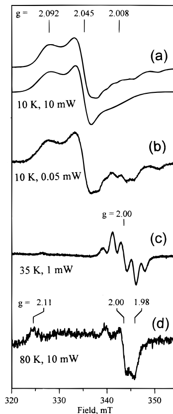
FIGURE 3: X-band EPR spectra of ferricyanide-oxidized native FTR. Native FTR ( 150 \mu\text{M} ) was prepared in 100 mM phosphate buffer, pH 7.6, and oxidized aerobically by incubation for 2 min with a 10-fold excess of potassium ferricyanide for spectra (a), (b), and (d) and with a 100-fold excess of potassium ferricyanide for spectrum (c). EPR conditions: temperature and microwave power, as indicated; modulation amplitude, 0.63 mT; microwave frequency, 9.60 GHz. The lower spectrum in (a) is a simulated powder EPR spectrum with g = 2.092, 2.045, and 2.008 , with line widths of 7.7, 3.8, and 11.5 mT, respectively.
