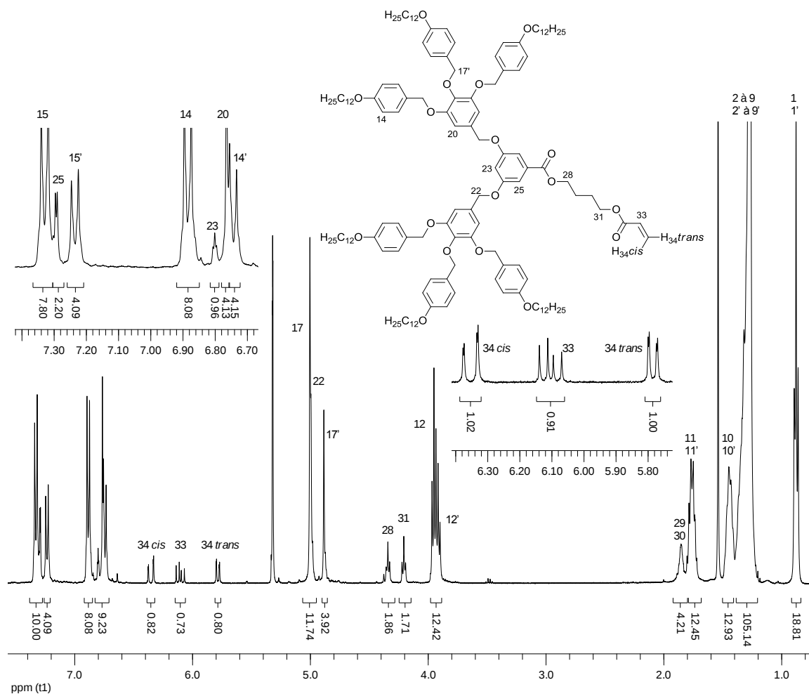
Figure 59. Spectre ^1\text{H} -RMN (400 MHz, \text{CD}_2\text{Cl}_2 ) du composé 60.
