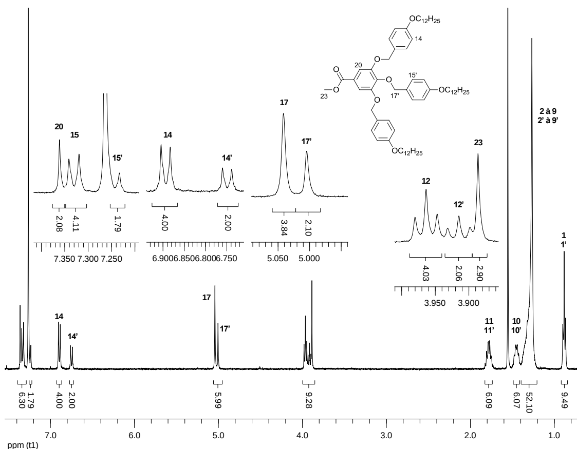
Figure 45. Spectre ^1\text{H} -RMN (400 MHz, \text{CDCl}_3 ) du composé 24 .
