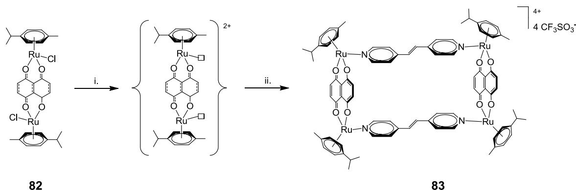
Schéma 38. i. \text{AgCF}_3\text{SO}_3 , MeOH ; ii. 1,2-bis(4-pyridyl)éthylène, MeOH, 60°C 24h, 73%.
