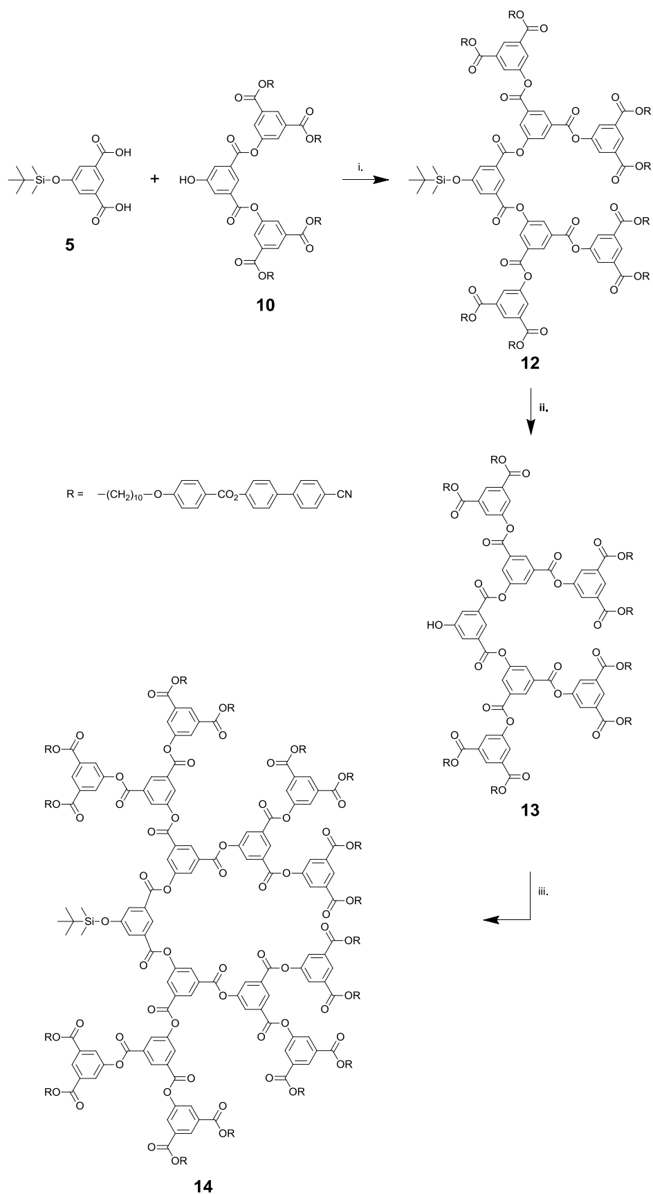
Schéma 7. i. DCC, DPTS, \text{CH}_2\text{Cl}_2 sec, t.a. 1 nuit, 90% ; ii. \text{Zn}(\text{BF}_4)_2 \cdot 6\text{--}7 \text{ H}_2\text{O} , THF/ \text{H}_2\text{O} (5/1), 50^\circ\text{C} 20h, 78% ; iii. DCC, DPTS, 4-ppy, \text{CH}_2\text{Cl}_2 sec, t.a. 2 jours, 90%.
