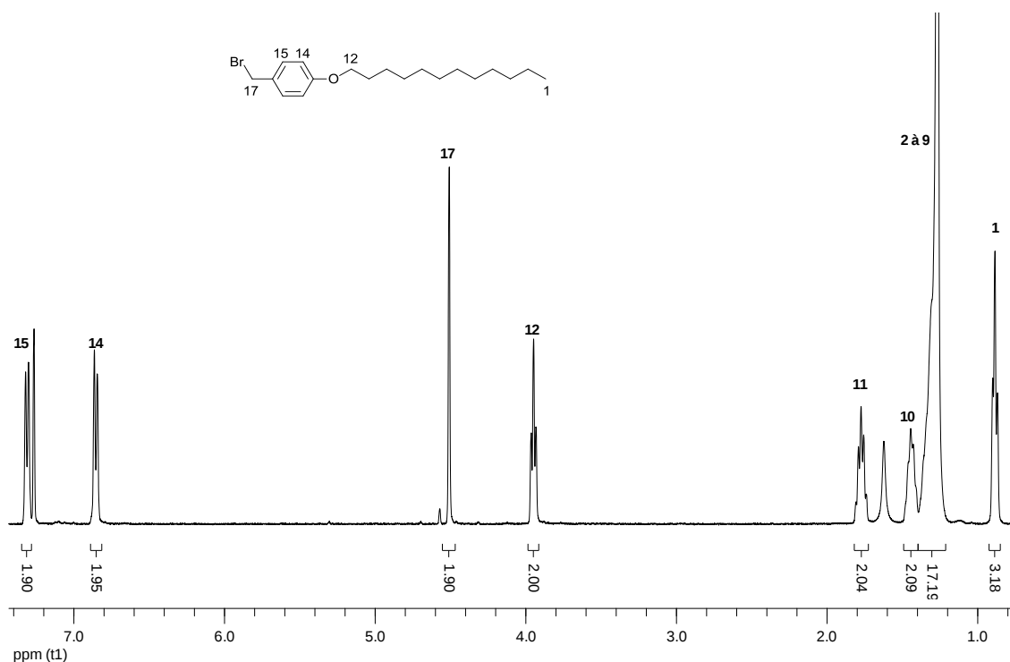
Figure 44. Spectre ^1\text{H} -RMN (400 MHz, \text{CDCl}_3 ) du composé 23 .
