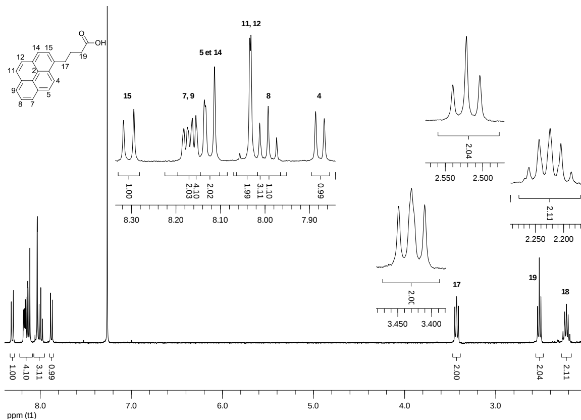
Figure 36. Spectre ^1\text{H} -RMN (400 MHz, \text{CDCl}_3 ) de l'acide 1-pyrènebutyrique.
