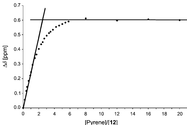
Fig. 7. ^1\text{H-NMR} Chemical-shift changes \Delta\delta ( 25^\circ , \text{CD}_3\text{CN} ) of the \text{H} -atoms of the ethenediyl moiety of 12 upon addition of pyrene to 12
