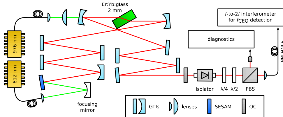
Fig. 1. Overview of the laser setup, consisting of a 2-mm thick Er:Yb:glass gain material pumped at 976 nm, 10 GTI mirrors with a total GDD of -1000 \text{ fs}^2 , a SESAM, and a 1.7% OC. Additionally, the SESAM is pumped with an 812-nm cw pump laser, which is not part of the actual laser cavity. This is indicated as a green line at the bottom left of the figure.
