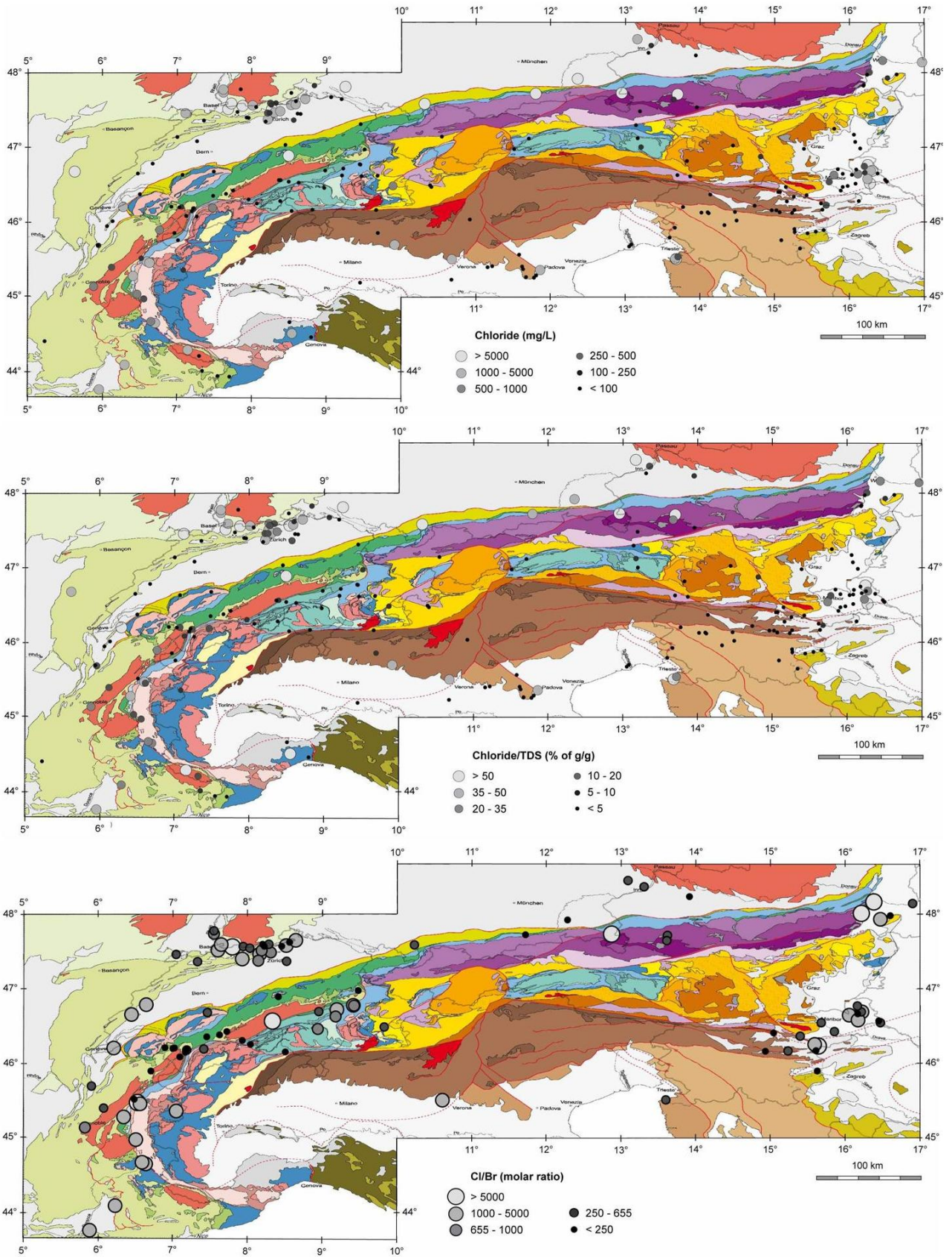
Plate 2: Maps of chloride contents, Chloride/TDS and Cl/Br ratios for the deep fluids in the Alps. Due to the lower density of the Cl/Br points, symbols are shown larger.
