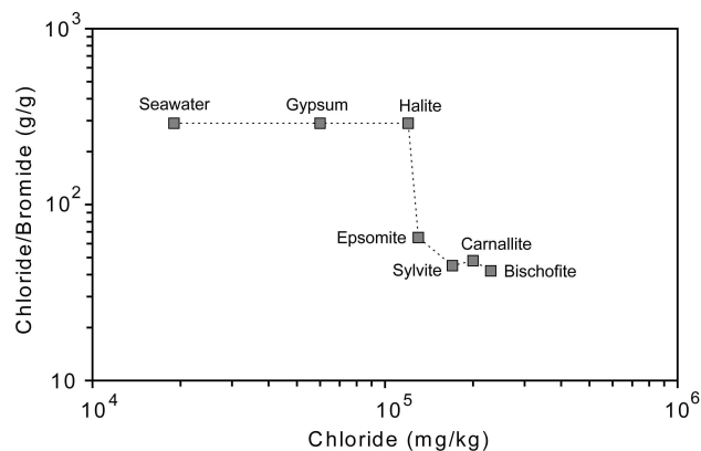
Figure 1: Cl/Br vs. Cl plot for residual brines formed during the successive phases of seawater evaporation (modified from Fontes and Matray, 1993)
