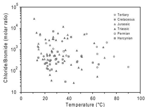
Figure 5: Cl/Br ratios vs. temperature for the deep fluids in the Alps and neighbouring areas. All data are listed in table 1.
