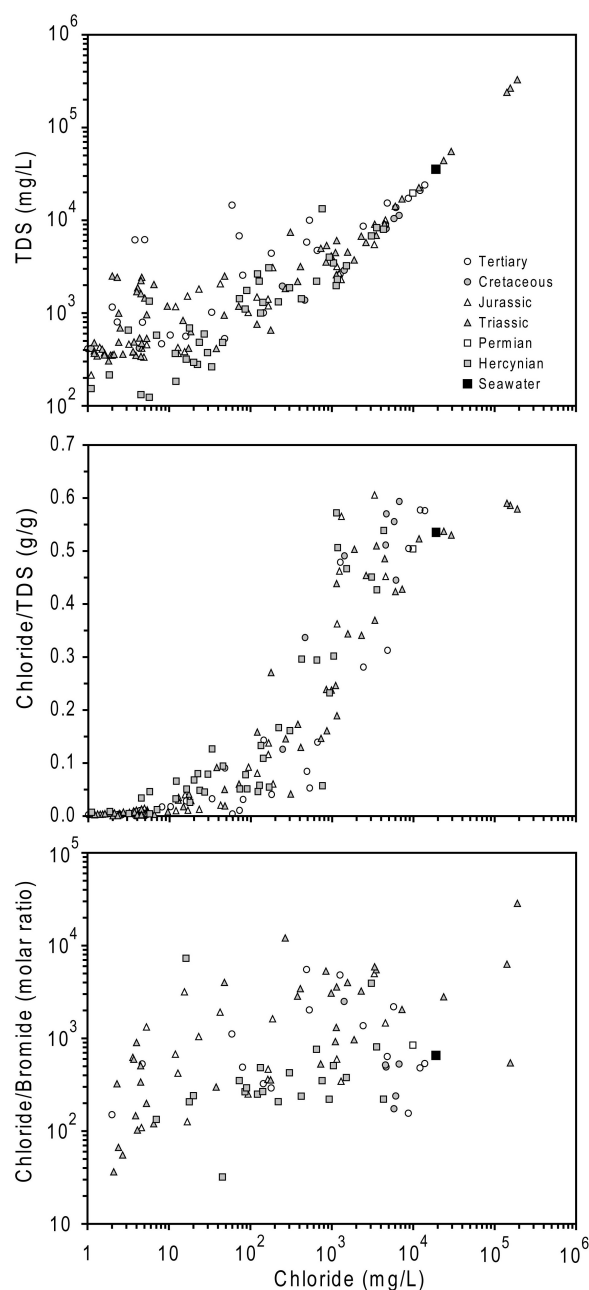
Figure 3: TDS, Chloride/TDS and Cl/Br ratios vs. chloride for the deep fluids in the Alps and neighbouring areas. All data are listed in table 1.
