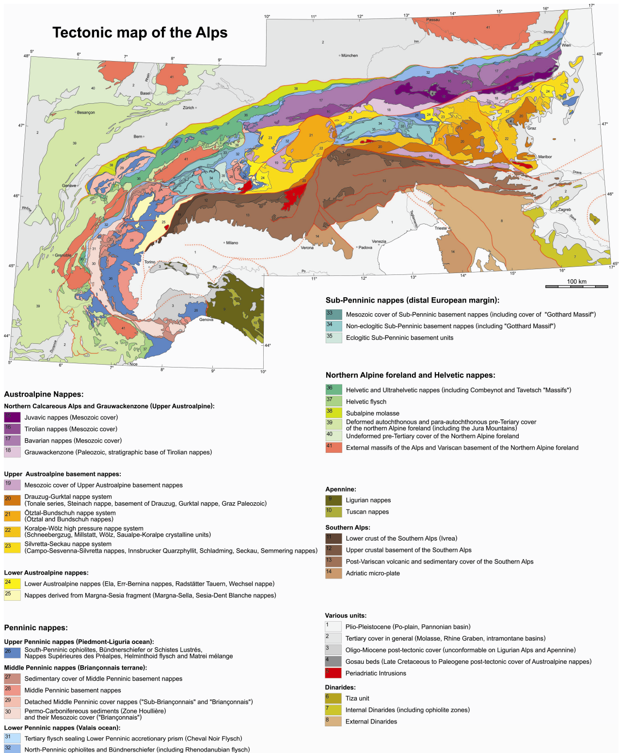
Plate 1: Tectonic map of the Alps range (Schmid et al., 2004).
