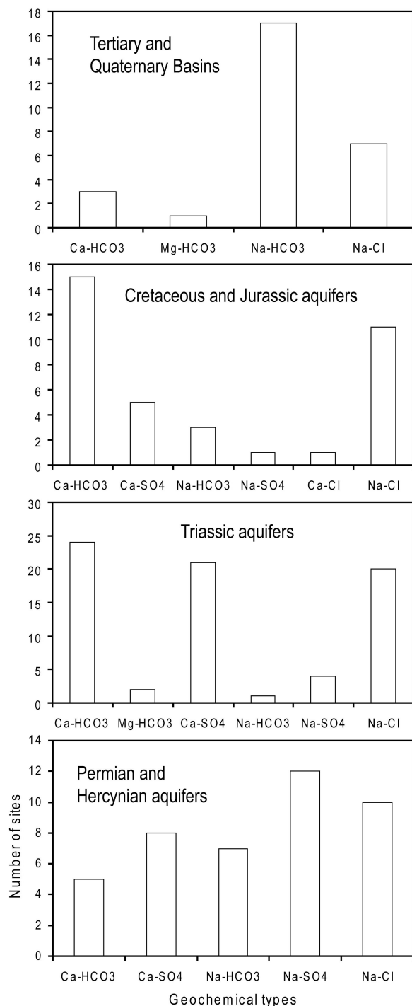
Figure 4: Histograms of geochemical types for deep fluids in various geological settings in the Alps and neighbouring areas.
