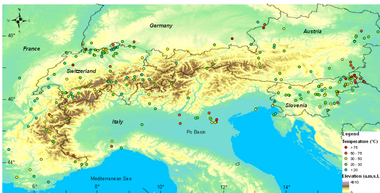
Figure 2: Locations of hydrothermal sites in the Alps range and neighbouring areas.
