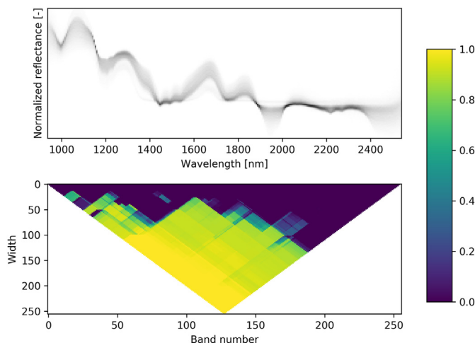
Fig. 8. Accuracy of classification of gypsum spectra, depending on the spectral area which is provided to the ANN. Similarly to Fig. 7, we can observe that the relevant part of the spectrum is the lowest wavelengths. This matches our intuition since it's the part of the spectrum with distinctive shape.
