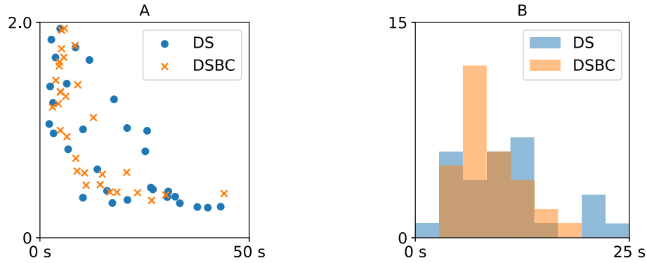
Fig. 4. Simulation time of a single realization versus the total error \epsilon_c (A). Histogram of \text{time} \times \epsilon_c (B).
