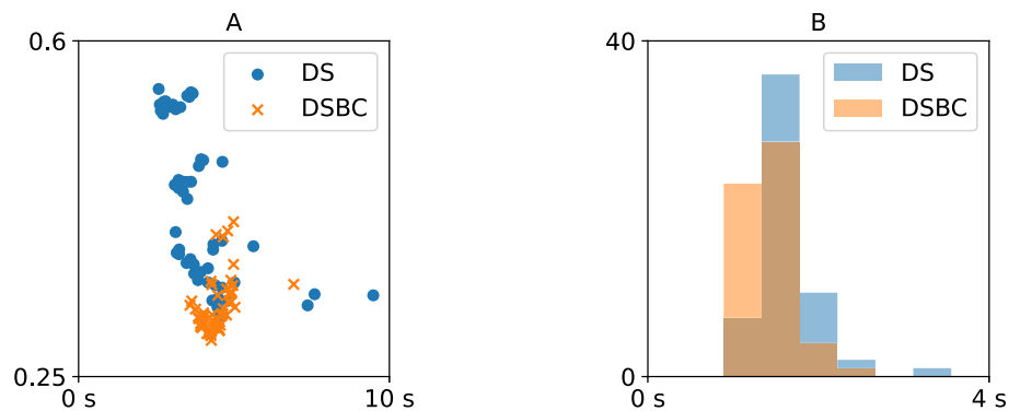
Fig. 11. Simulation time for Case 3 of a single realization versus the CV loss (A). Histogram of \text{time} \times \text{CV loss} (B).
