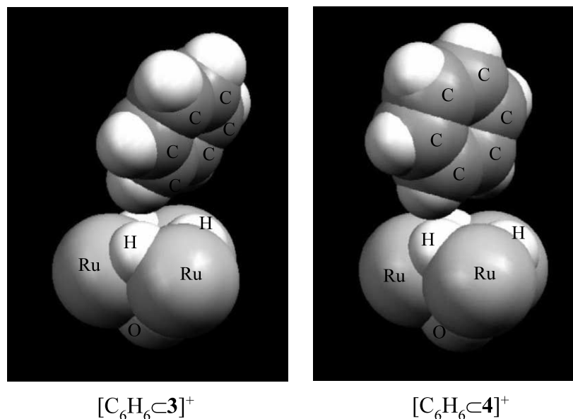
Fig. 6. Space filling representation of the host-guest complexes [\text{C}_6\text{H}_6 \subset \mathbf{3}]^+ and [\text{C}_6\text{H}_6 \subset \mathbf{4}]^+ with the benzene guest (top) approaching the \text{Ru}_2 plane, the arene ligands being omitted for clarity.
