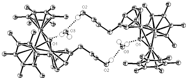
Fig. 3. Hydrogen-bonded dimers of [C_6H_6\text{-}c\text{-}4][BF_4]\cdot H_2O\cdot 0.5C_6H_6 .
