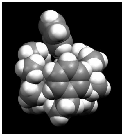
[C_6H_6\text{-}c\text{-}3]^+
