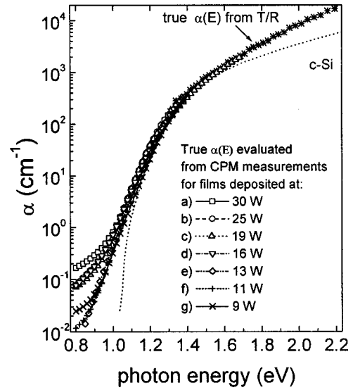
FIG. 7. Comparison of the true optical absorption coefficient \alpha_{\text{true}} for a series of \mu\text{c-Si:H} films prepared at different discharge powers and at dilution of silane in hydrogen of 5%.
