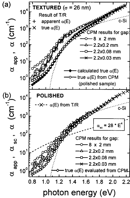
FIG. 6. Apparent optical absorption coefficients of sample B measured by CPM with different interelectrode spacing (gap) and calculated from T/R measurements: (a) in the as-grown state (textured sample) and (b) after a chemomechanical polishing and H_2 plasma treatment. The evaluated spectral dependence of the true absorption coefficient \alpha(E) is shown as the main result by solid or empty diamonds; \alpha(E) of crystalline silicon is shown for comparison. The rms surface roughness \sigma=26 nm of the as-grown sample was evaluated from the T/R data.
