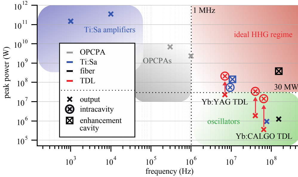
Fig. 1. Overview of peak power and repetition rate of some representative laser systems, including Ti:Sapphire (Ti:Sa) amplifiers [13, 14] and oscillators [15], fiber amplifiers [16], OPCPA systems [17, 18], as well as parameters typically reached inside enhancement cavities [6, 19]. The ideal laser parameters zone for megahertz high-harmonic generation (HHG), e.g. in a gas target, is marked as red-shaded area ( f_{\text{rep}} > 1 \text{ MHz} , P_{\text{peak}} > 30 \text{ MW} ). In this graph, the trade-off between repetition rate and peak power of currently existing state-of-the-art systems is clearly illustrated. For some current thin disk laser (TDL) results [10, 20, 21], both extra- and intra-cavity parameters are marked in red crosses and crossed circles respectively. Stabilized high-average power frequency combs from TDLs look promising and could also be combined with external pulse compression to further increase the peak power [22].
