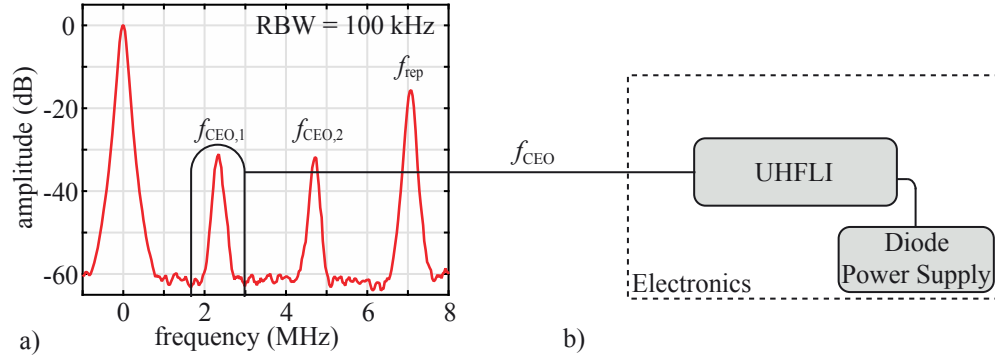
Fig. 7. a) Microwave spectrum of the Yb:YAG laser measured at the output of the f -to- 2f interferometer, showing f_{\text{CEO},1} and f_{\text{CEO},2} around 2.33 MHz and 4.67 MHz, respectively, for f_{\text{rep}} = 7 MHz. A resolution bandwidth (RBW) of 100 kHz is used here. b) Schematic of the electronic filtering and demodulation of the CEO beat in the Yb:YAG laser using only the UHFLI in order to perform characterization on the f_{\text{CEO}} signal and to apply signal on the pump diode to modulate its current.
