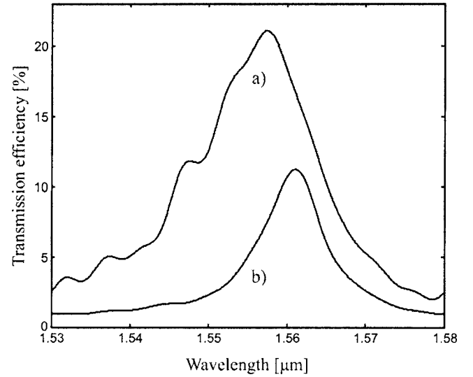
FIG. 4. Measured transmission spectrum of (a) a four-hole reflector cavity and (b) a five-hole reflector cavity. The raw measurement data have been filtered to remove the Fabry-Pérot interference.
