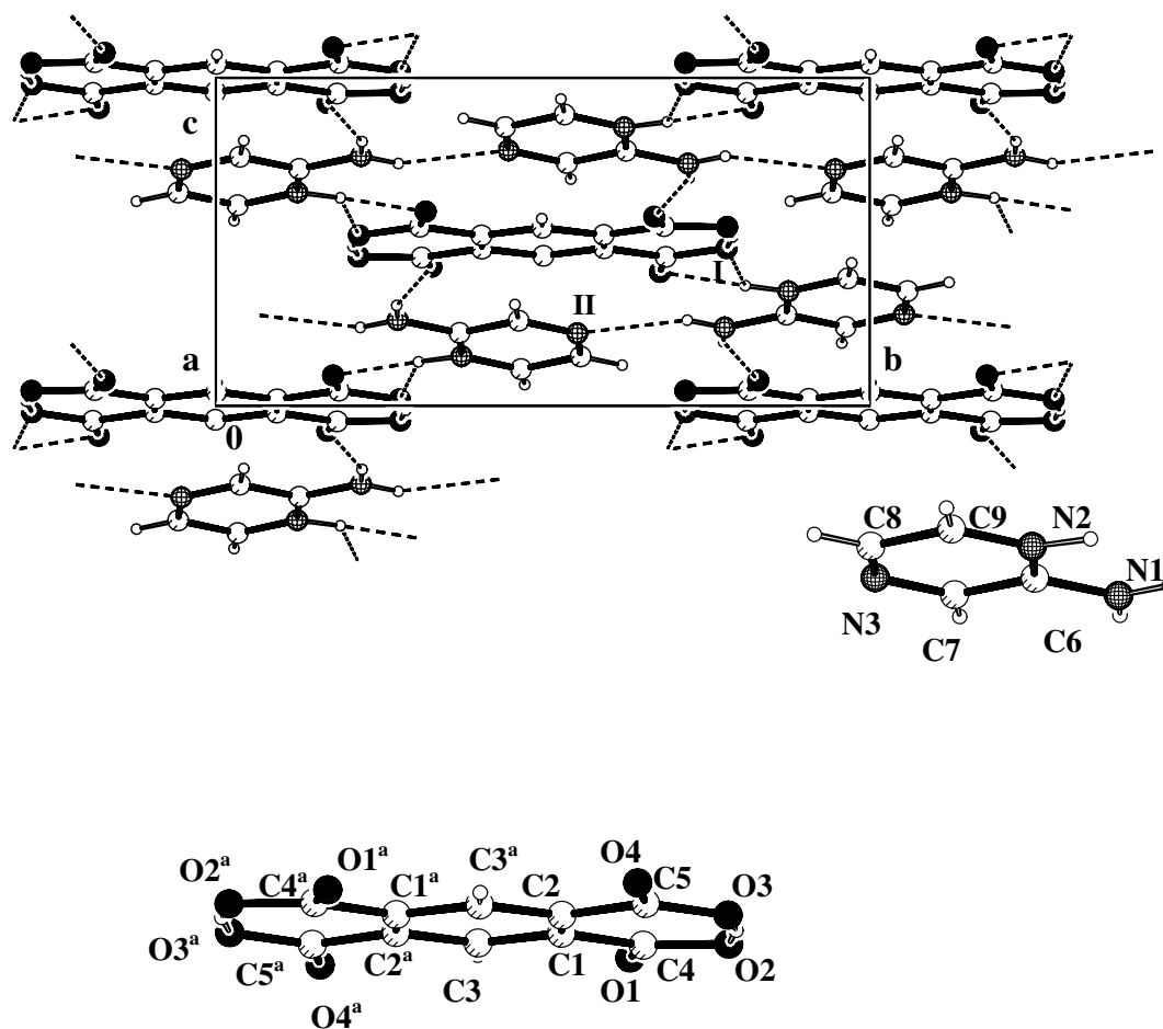
Figure 4.5 Crystal packing diagram for organic salt [(H 2 -BCTA)(H-Apyz) 2 ]; a ) 1- x , - y , - z . Ring motifs (I): R 1 2 (4), (II): R 3 3 (17).
