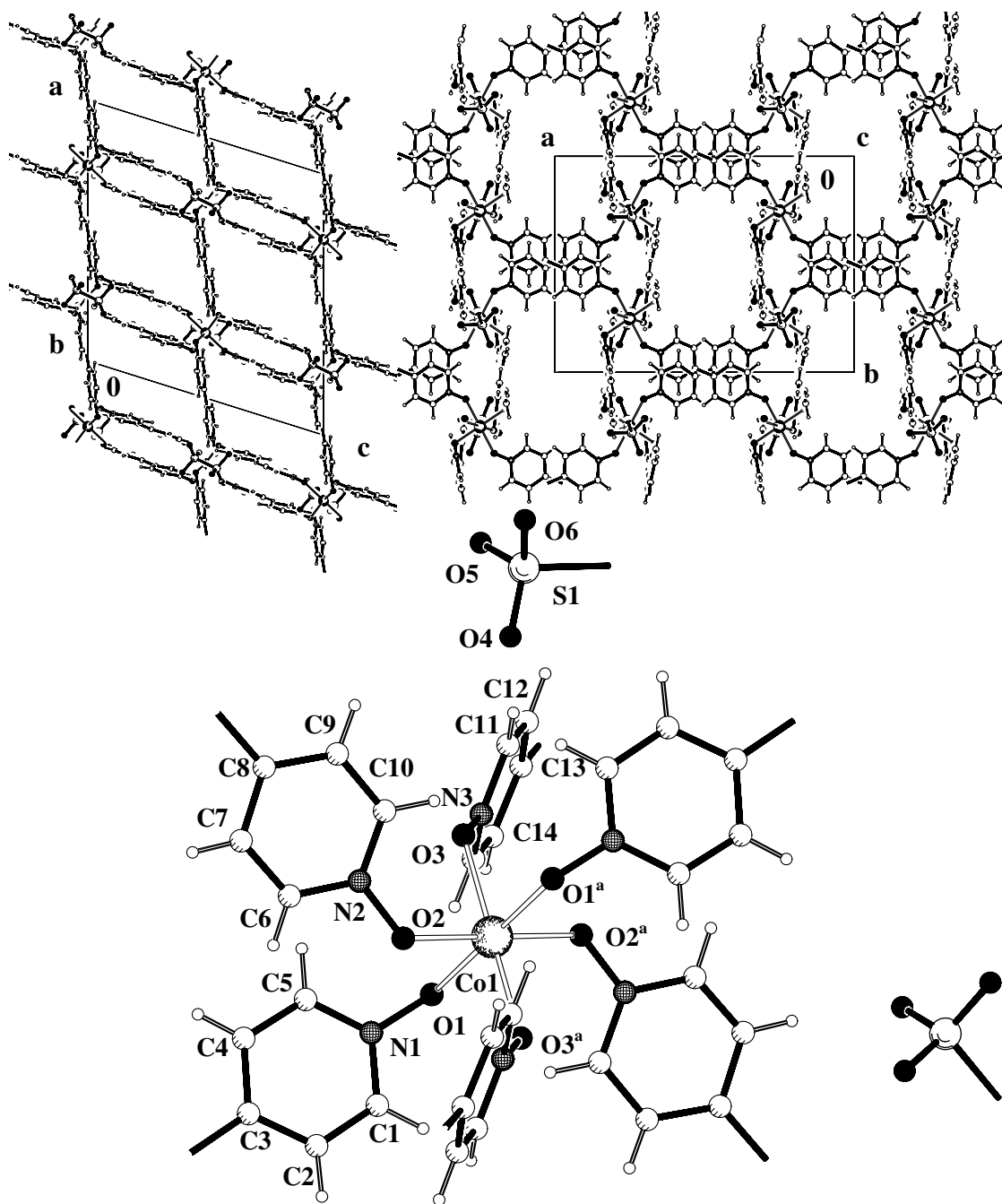
Figure 3.3 Crystal packing diagrams and Co II coordination sphere for complex C16 ; a ) 1/2- x , 1/2- y , 1- z
