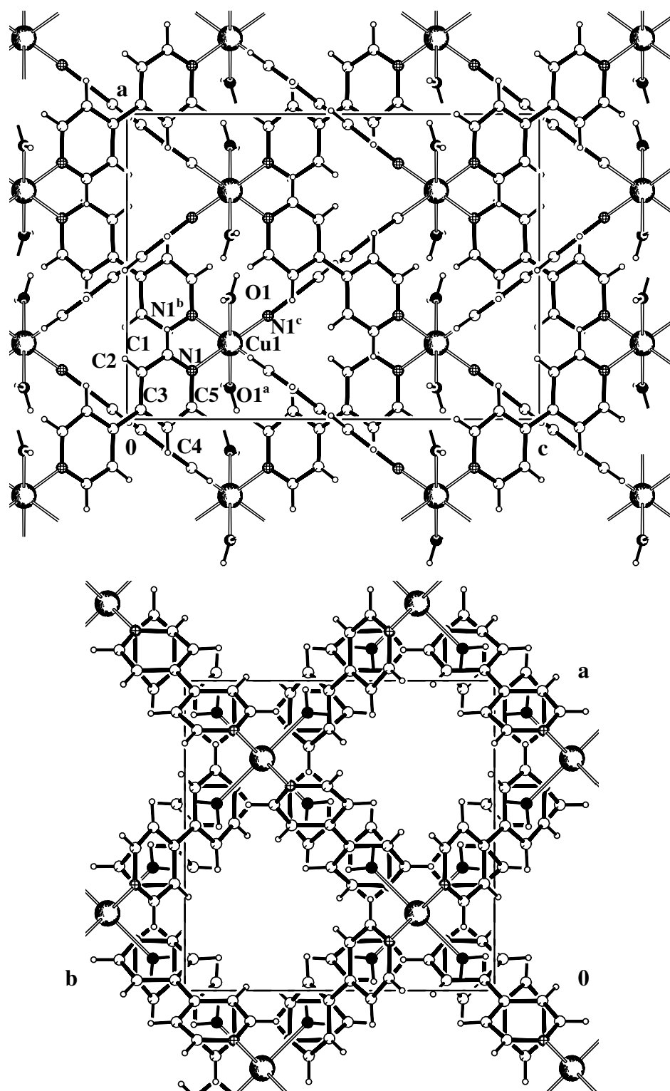
Figure 2.15 Crystal packing diagrams of C9 (the strongly disordered \text{S}_2\text{O}_6^{2-} anions are omitted for clarity); a ) 3/2-x, 1/2-y, z , b ) 1/2+y, -1/2+x, 1/2-z , c ) 1-y, 1-x, 1/2-z
