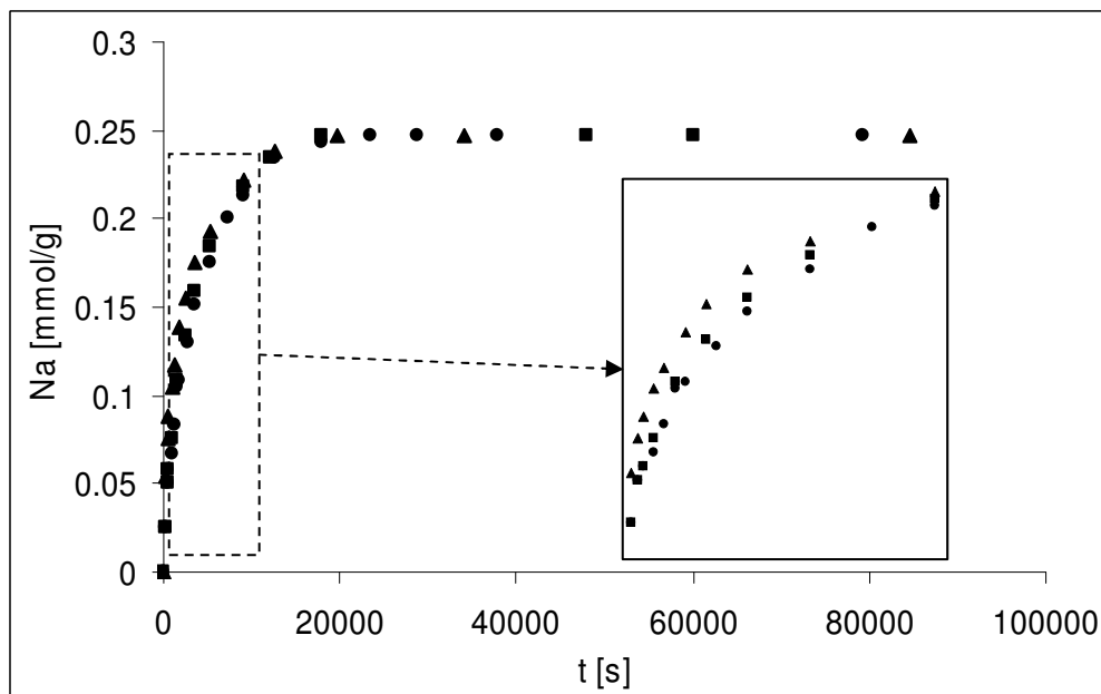
Figure 2.37 Kinetic studies for CH 2 Cl 2 adsorption on C11 at 293 K (●), 301 K (■) and 308 K (▲).
