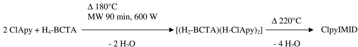
Reaction 4.3
