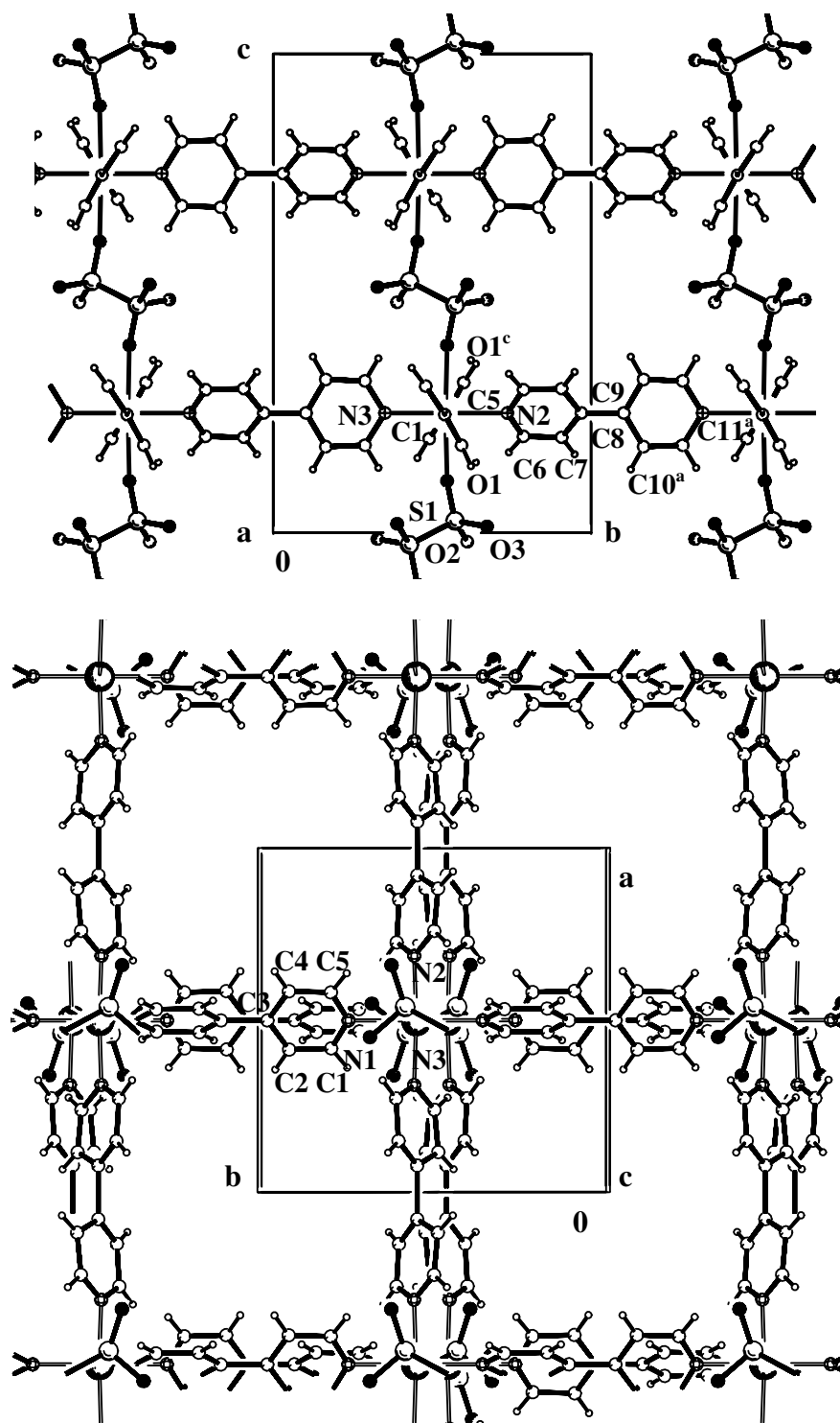
Figure 2.14 Crystal packing diagrams of complex C8 ; a ) x, -1+y, z c ) 1-x, y, 3/2-z
