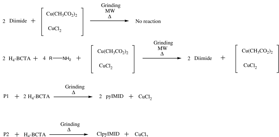
Scheme 4.4 Complexation tests
