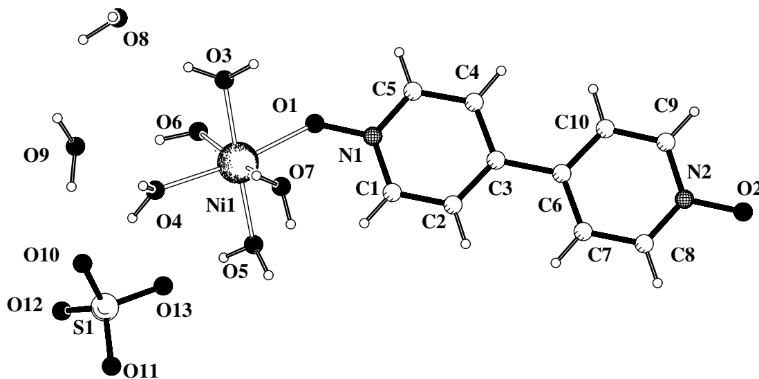
Figure 3.9 \text{Ni}^{\text{II}} coordination sphere for complex C19
