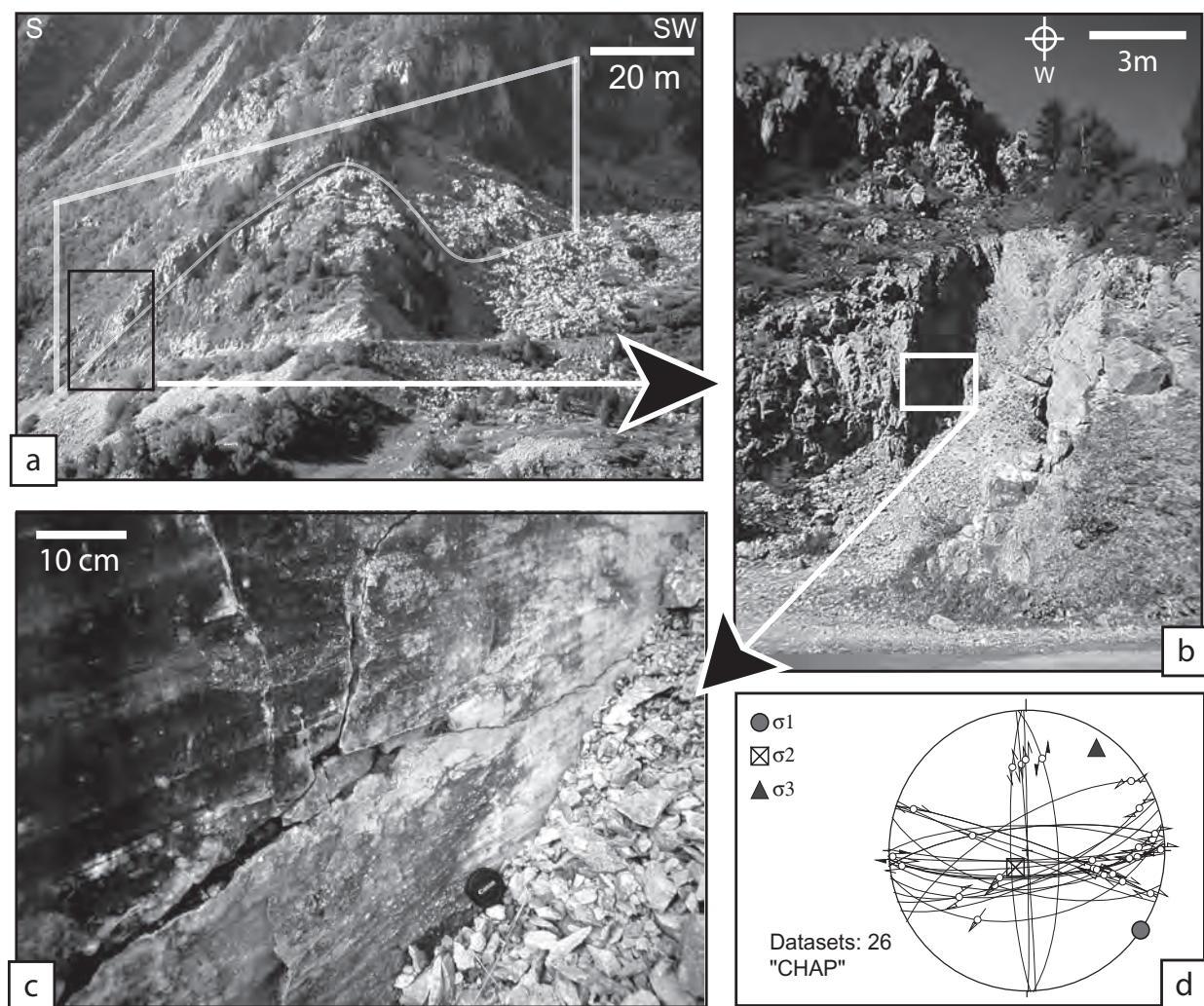
Fig. 2 (a) Morphological expression of a kilometric length fault (the ‘Chapieùx–Roseland’ Fault viewed from the north). The movement along the nearly vertical fault plane is transcurrent. (b) Outcrop-scale view of the same fault. The fault plane is vertical, and associated with a thick fault gouge (about 4 m). This tectonic clay is the expression of a large amount of displacement, under conditions of low temperature and low fluid pressure, probably close to the surface. (c) Small-scale observation of the same fault shows a very slick fault plane, with horizontal and curved mechanical scratches. The fault plane cross-cuts an older cataclasite, with millimetric to centimetric broken then consolidated elements. There is no mineralization on the plane. (d) Measurements of several fault planes in this sector allow us to calculate the local palaeostress tensor. The major fault belongs to an east–west fault family, conjugated with a north–south more discrete fault family. The calculated tensor indicates a transcurrent stress field, with a N35° orientated \sigma_3 and N125° orientated \sigma_1 .
