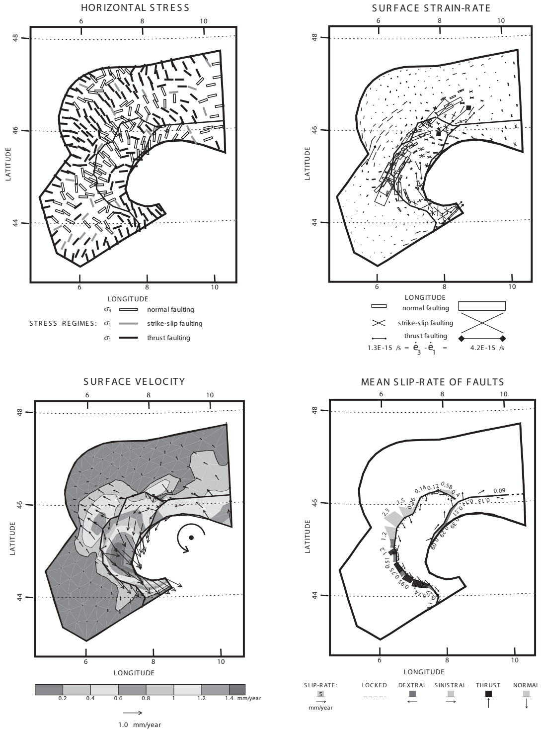
Figure 7: Model D. Model with realistic 3D crustal geometry and rotational Po plain boundary nodes. See Figure 5 for comparisons. Differences between models B and D are only due to rotational Po plain boundary (see text for explanation).
