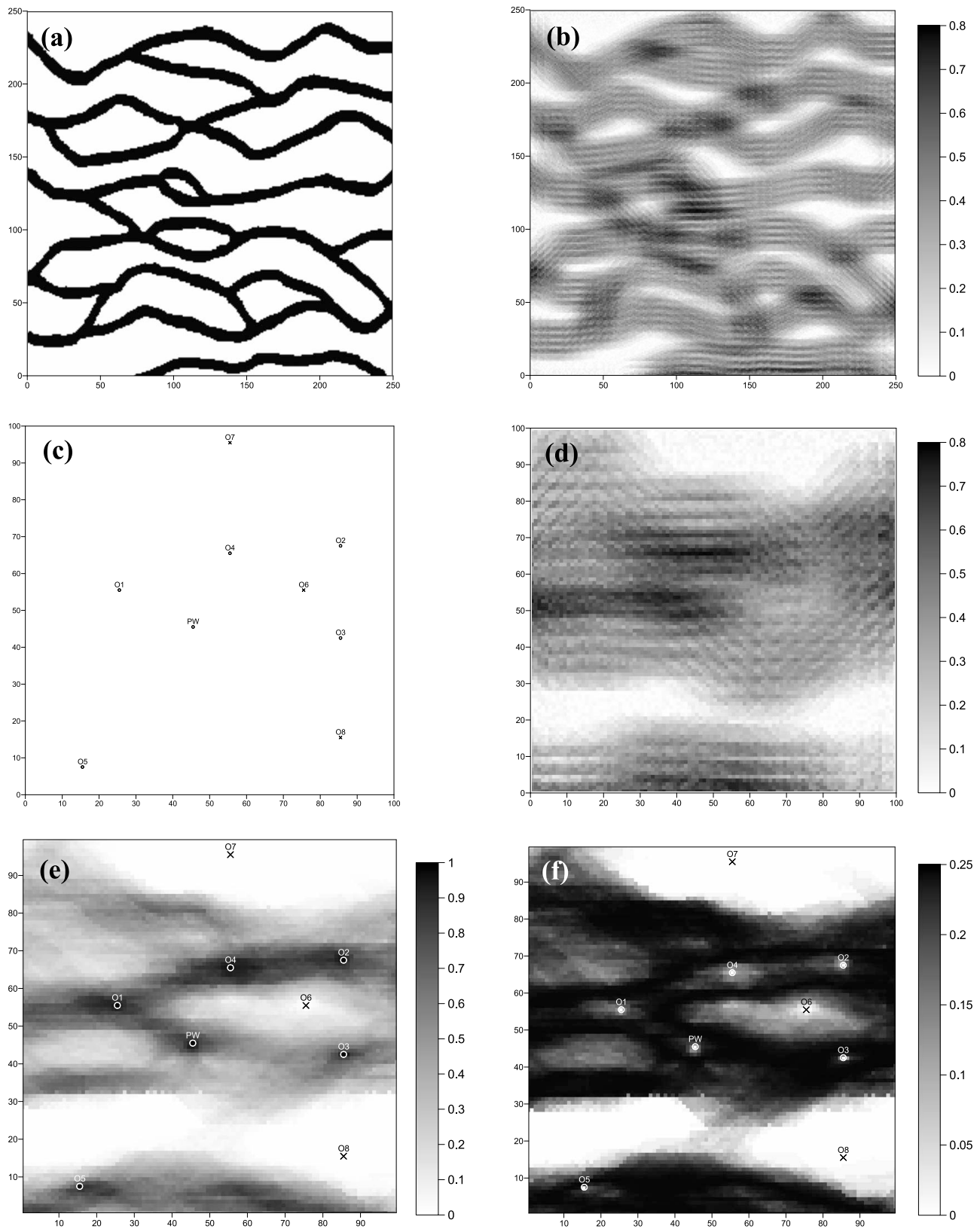
Figure 1. Geological setup. (a) Training image of the primary variable [Strebelle, 2002]. (b) Training image of the secondary variable (seismic data). (c) Measurement locations at sand and shale lithofacies (circles and crosses, respectively). (d) Exhaustive seismic data. (e) Ensemble mean of 100 plausible simulations. (f) Corresponding ensemble variance.
