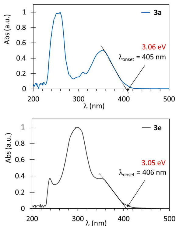
Fig. 5. UV–vis spectra of compounds 3a and 3e ( \text{CH}_2\text{Cl}_2 , 5 \cdot 10^{-5} M) with the respective band gap energy estimation.
