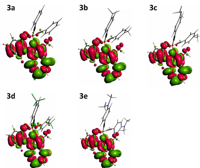
Fig. 10. Electron Difference Density Maps (EDDMs) for the lowest energy singlet electronic transition computed by TD-DFT (red indicates a decrease in electron density, green indicates an increase).
