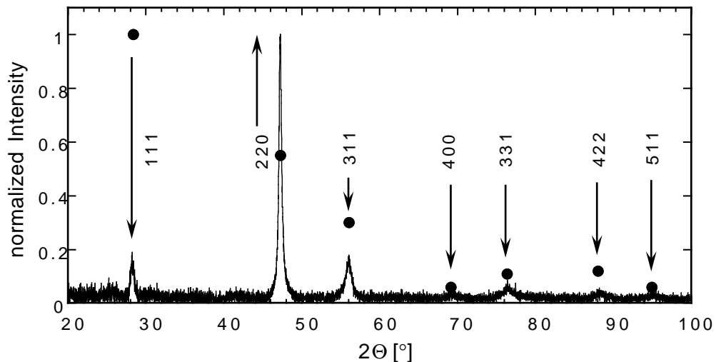
FIGURE 1. Typical X-Ray diffraction pattern of a \mu\text{c-Si:H} thin-film grown by VHF-GD deposition using Ar/H 2 dilution. The points refer to the powder sample according to the JCPDS (28).
