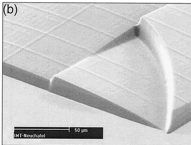
Fig. 7. Scanning-electron microscope image of the first element fabricated by HEBS glass gray-tone lithography in photoresist: (a) overview, (b) enlarged detail.
