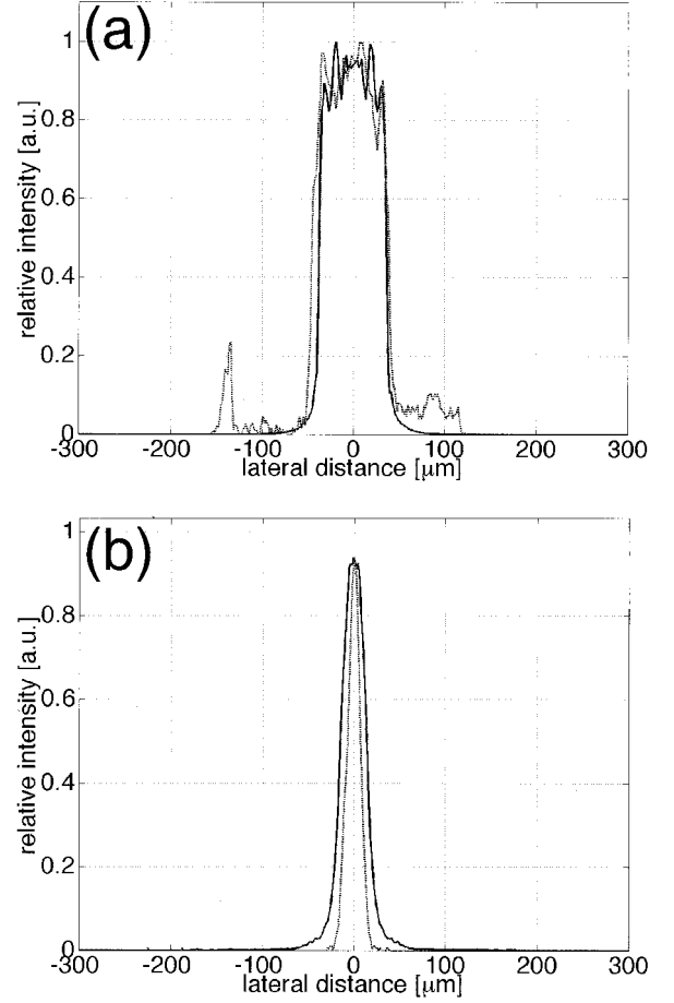
Fig. 6. Calculated and measured intensity distributions in the plane of the fiber: (a) cross section parallel to the slow axis of the diode laser, (b) cross section parallel to the fast axis of the diode laser. Solid curves, theory; dashed curves, experiment.
