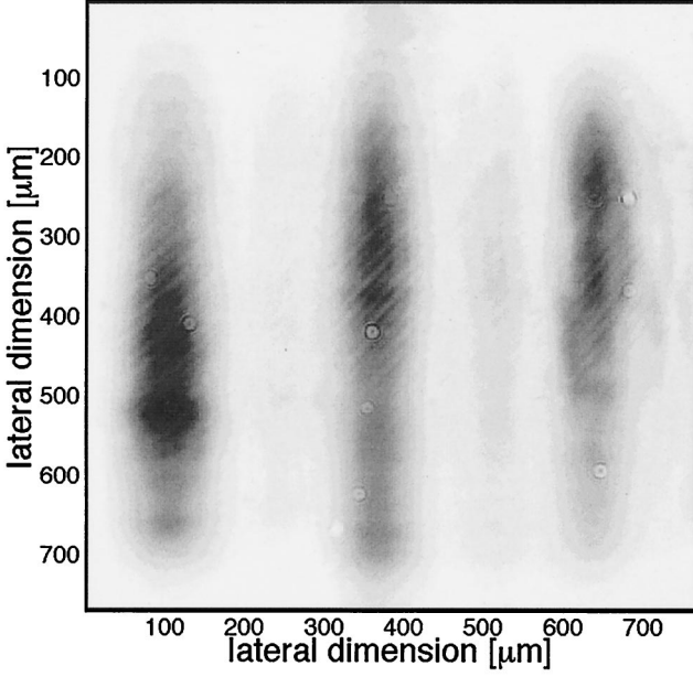
Fig. 3. Typical measured two-dimensional intensity distributions in the plane of the second DOE.
