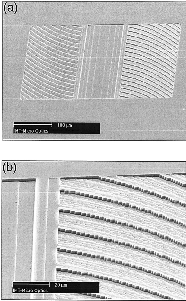
Fig. 9. Scanning-electron microscope image of the first element fabricated as a multilevel structure (eight levels) in fused silica: (a) overview, (b) enlarged detail.
