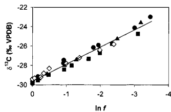
FIGURE 4. Rayleigh type plot for MTBE for microcosm enrichments 18-1 and 18-3 (filled circle), 8b-2i (filled square), 10a-2i (filled triangle), and cometabolic microcosm (open diamond). Line: Calculated isotope ratio using eq 2 and the average enrichment factor of all experiments. The uncertainty of the \delta^{13}\text{C} measurement corresponds approximately to the size of the marker.
