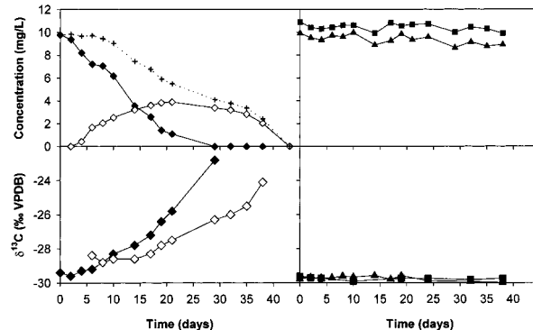
FIGURE 3. Left: Concentration and \delta^{13}C of MTBE (filled diamond) and TBA (open diamond) in microcosm with 3-methylpentane as primary substrate and sum of MTBE and TBA (cross-hair) in mg/L MTBE equivalent. Right: Concentration and \delta^{13}C of MTBE in sterile control (square) and microcosm with no cosubstrate (filled triangle). The uncertainty of the \delta^{13}C measurement corresponds approximately to the size of the marker.
