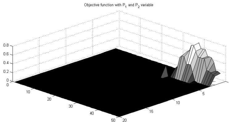
Figure 12: Objective function F for Casablanca data
