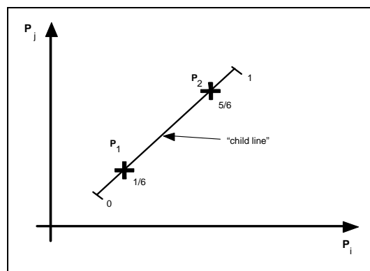
Figure 5: linear crossover process of the GA
