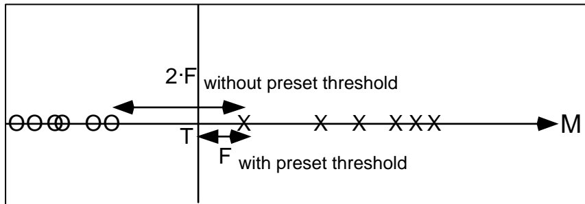
Figure 2: objective function for 1-dimensional measurement space
