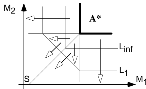
Figure 10: Gradients of the objective functions defined with L_1 and L_\infty metrics
