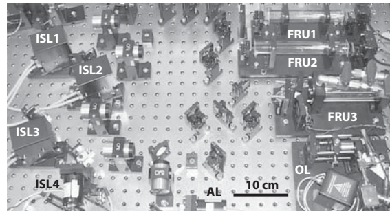
Fig. 6. Photograph of the realised FDU system. Left-hand side: the four ISL laser units. Right-hand side: the four frequency reference units (FRU1 to FRU4, from top to bottom). Middle part: transfer optics (optical isolators and beamsplitters) and additional fifth laser (AL) for test and characterisation purposes. The dimensions of the realised instrument are 75 x 53 x 15 cm 3 .
