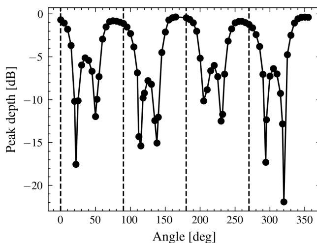
FIG. 8. Measured microwave mode peak depth with respect to the rotation angle between the microwave coupling loop and the cavity. See Fig. 3 for the 0^\circ reference position. Given the angle, coupling to the mode of interest can be either enhanced or depleted.
