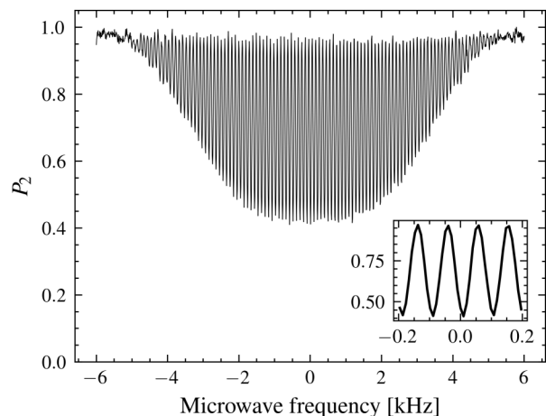
FIG. 11. Ramsey fringes for T_R = 10 ms and t_m = 167 \mu\text{s} . The main figure and the inset share the same axes.
