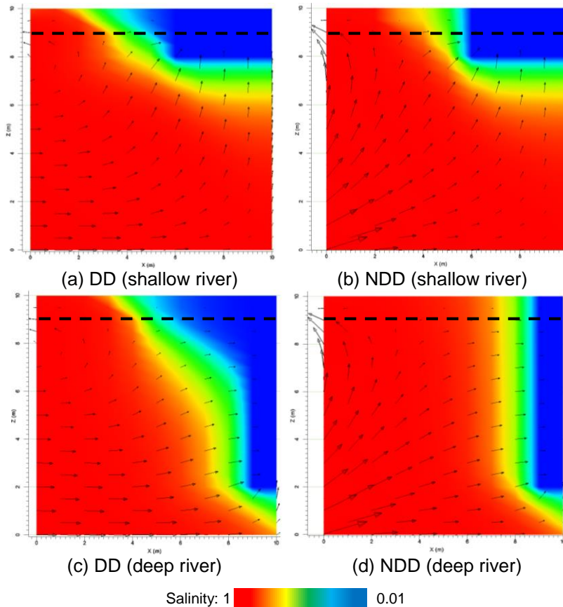
Figure 8. Simulated salinity distribution in the small scale model for river dimension scenario (RD). Dotted black line represent the groundwater table.
