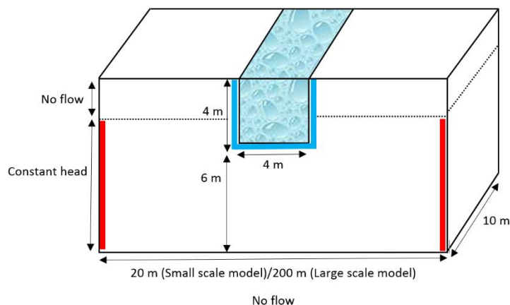
Figure 1. Conceptual model with boundary conditions and dimensions. The dimensions and boundary conditions are symmetrical. Note that the figure is not drawn to scale. Fresh and saline solute transport boundary conditions are shown in blue and red, respectively.
