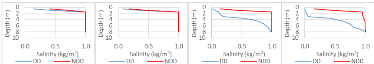
Figure 4. Groundwater salinity profile at the location of observation wells.
