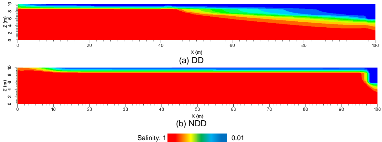
Figure 2. Simulated salinity distribution in the large scale model for Scenario BC.
