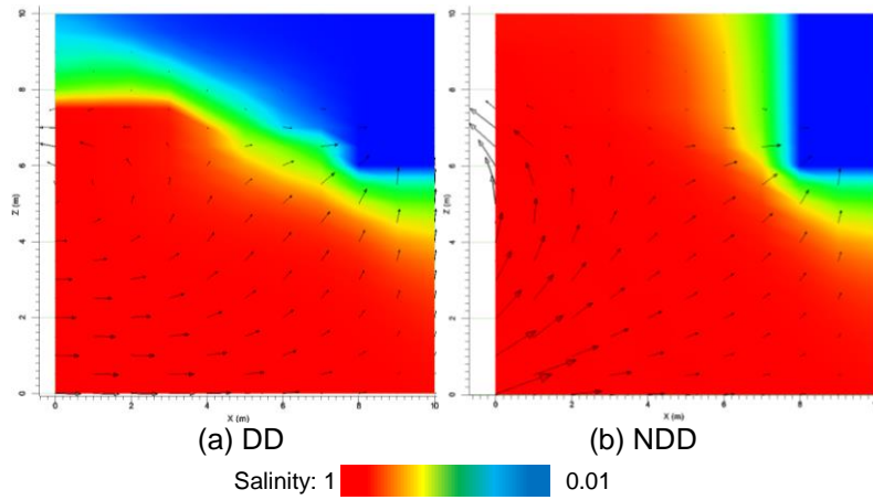
Figure 5. Simulated salinity distribution in the small scale model for base-case scenario (BC). Dotted black line represents the groundwater table.
