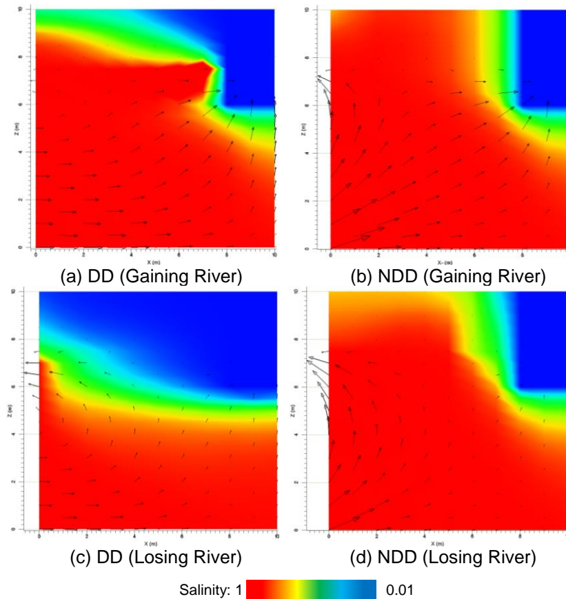
Figure 7. Simulated salinity distribution in the small scale model for gaining and losing scenario.
