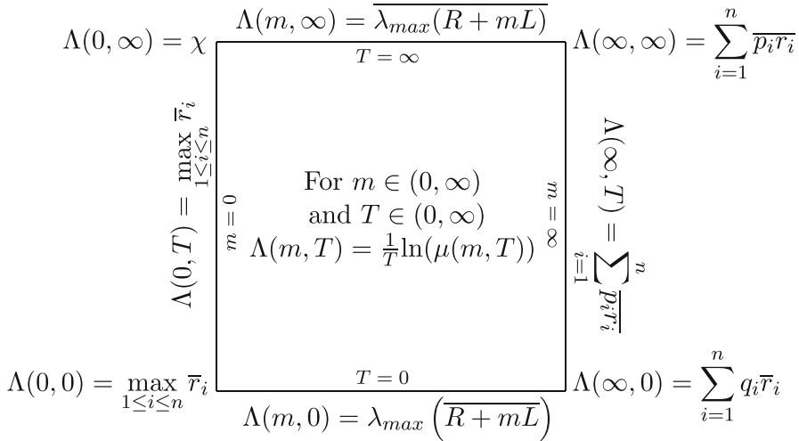
Fig. 1 The definition of \Lambda(m, T) and its limits when T tends to 0 or \infty and/or m tends to 0 or \infty
