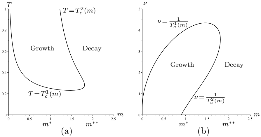
Fig. 6 a The set \Lambda(m, T) = 0 . b The set \Lambda(m, \nu) = 0 . The parameter values are those of (61). We have m^* \approx 0.904 and m^{**} \approx 1.807
