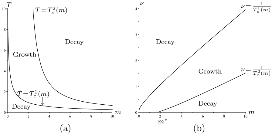
Fig. 5 a The set \Lambda(m, T) = 0 . b The set \Lambda(m, \nu) = 0 . Here we use the parameter values of (58) ( m^* = 1.764 )
