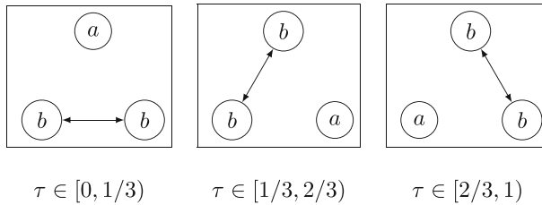
Fig. 8 The three-patch model
