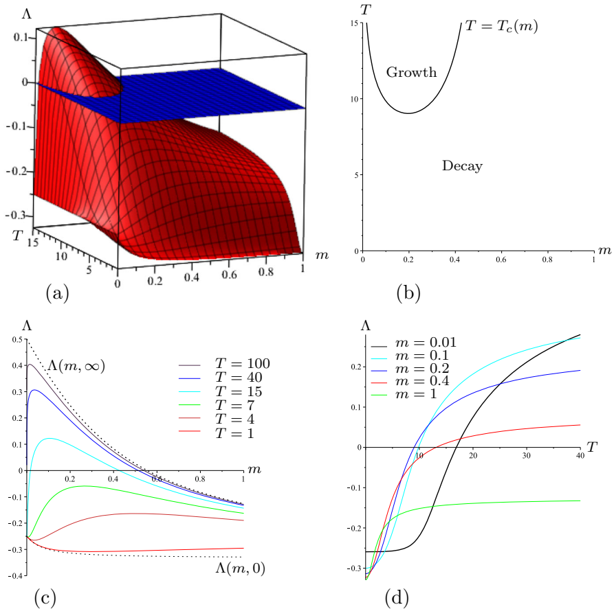
Fig. 2 a The graph of (m, T) \mapsto \Lambda(m, T) . b The set \Lambda(m, T) = 0 . c Graphs of m \mapsto \Lambda(m, T) with the indicated values of T . d Graphs of T \mapsto \Lambda(m, T) with the indicated values of m . Here we used the two patch model corresponding to the matrices (52) and \alpha = 0.5
