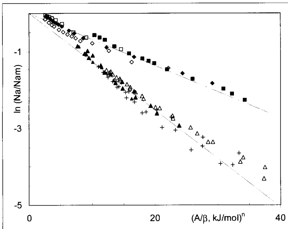
Fig. 2. The adsorption of N_2 (77 K) on Cabosil , (■); Fransil (□), Nucleosil-300 (◇) and Nucleosil-1000 (◆); C_6H_6 (293, 303, 313 K) (▲), CH_2Cl_2 (293, 313 K) (△) and CCl_4 (293, 310 K) (+) on Cabosil ; CCl_4 (293 K) (+) on Fransil . For nitrogen exponent n = 1.8 and E_{N_2}(77\text{ K}) = 4.62\text{ kJ mol}^{-1} . For the other adsorbates n = 1.2 and E_{C_6H_6} = 5.61\text{ kJ mol}^{-1} .
