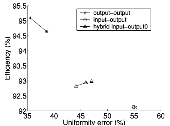
Fig. 7 Comparison of the results of the three variants of Fienup's algorithm, namely input-output, output-output, and hybrid output-output.
