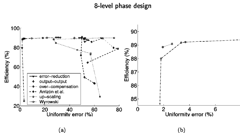
Fig. 5 Comparison of efficiency and uniformity error of an 8-level profile design with various algorithms; (b) is a magnification of (a).
