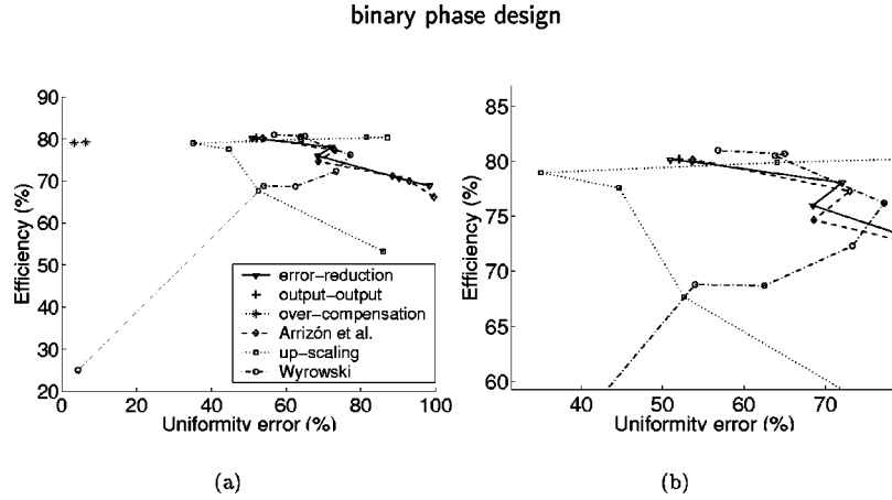
Fig. 6 Comparison of efficiency and uniformity error of a binary profile design with various algorithms; (b) is a magnification of (a).
