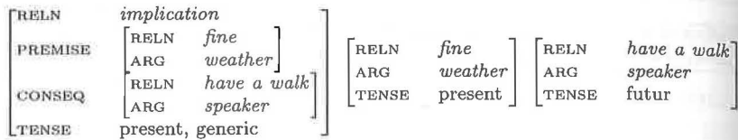
FIGURE 4 Information structure
