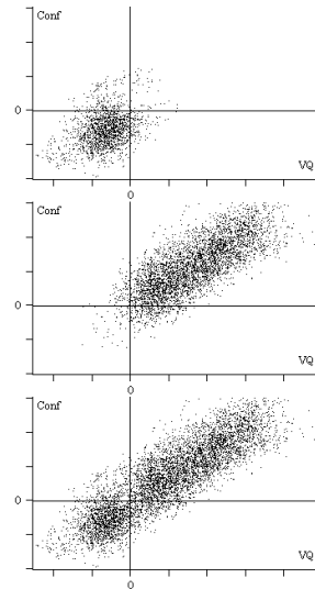
Figure 9: Scatter diagrams \langle VQ_c \rangle - \langle Conf_c \rangle . The first diagram shows the intra-speaker domain and the second diagram shows the inter-speaker domain. In the third and last diagram, the size of the intra-speaker dots is made larger in order to permit the comparison of the two domains. The distances are translated by the subtraction of the associated thresholds, which explains the appearance of negative distances.
