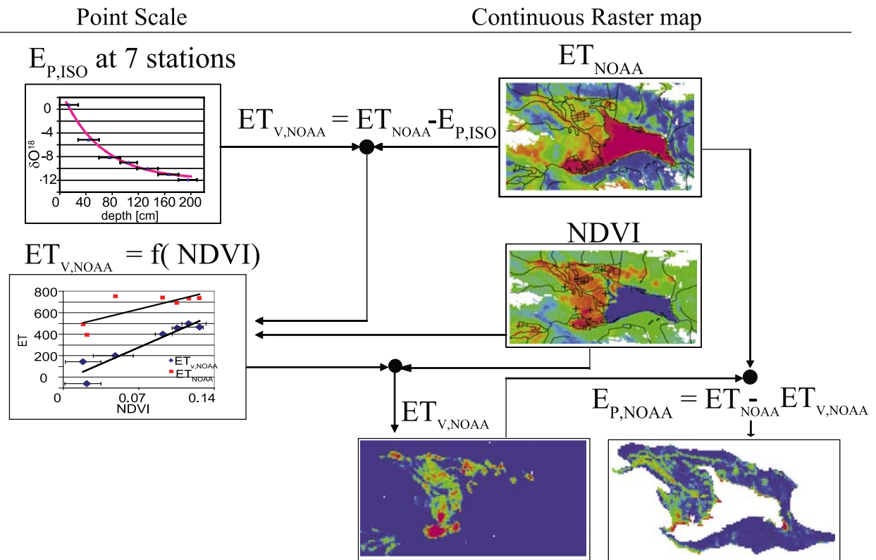
Figure 1. Schematic overview of calculation of phreatic evaporation. E_{P,ISO} is the phreatic evaporation rate calculated on the basis of stable isotopes. The values obtained by using this method represent a long-term average rather than an instantaneous value. ET_{NOAA} is defined as the total annual evapotranspiration rate based on the NOAA-AVHRR images. This annual value is calculated by extrapolating between several daily estimates of ET. ET_{V,NOAA} is the vadose ET rate obtained by the combination of ET_{NOAA} and E_{P,ISO} . The NDVI is the normalized differential vegetation index. The NDVI represents an annual average. E_{P,NOAA} is the phreatic evaporation rate, calculated by the combination of ET_{V,NOAA} , the NDVI, and ET_{NOAA} .
