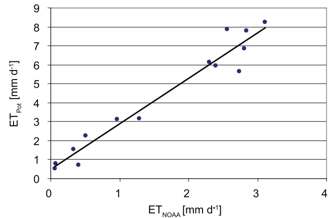
Figure 4. Comparison between the average ET estimates based on remote sensing ( ET_{\text{NOAA}} ) and the potential ET rates ( ET_{\text{Pot}} ) for Korla for the days NOAA-AVHRR images were available. The total annual ET calculated by using the Penman-Monteith equation is 1.4 \text{ m a}^{-1} .
