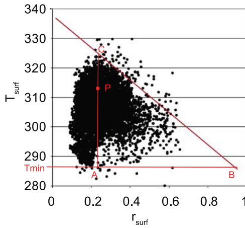
Figure 3. Feature space plot between albedo r_{\text{surf}} (Kelvin) and temperature T_{\text{surf}} (Kelvin) for an image over the project area (image date 27 April 2000).
