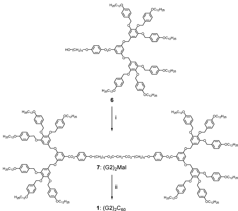
Scheme 1 (i) Malonyl chloride, Et 3 N, CH 2 Cl 2 , r.t., overnight, 27%; (ii) C 60 , DBU, I 2 , toluene, r.t., overnight, 26%. For abbreviations, see ref. 13.
