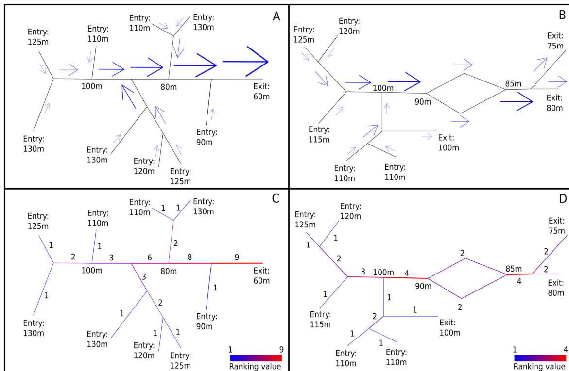
Fig. 9. A: Example of a branchwork network which could correspond to a fluvial network or a karstic network. The blue arrows show the direction of the flow and its size is proportional to the theoretical flow value. B: Example of complex network, with one loop and two exits, which could correspond to a karstic network. C-D: Proposed ranking method (top view) applied, respectively, to networks A and B.
