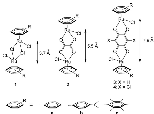
Figure 2. Dinuclear arene ruthenium building blocks.
