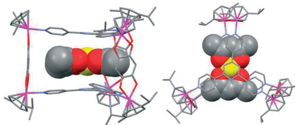
Figure 12. Molecular structure of [ (acac)_2Pt \subset 17b ] 6+ . [32]
