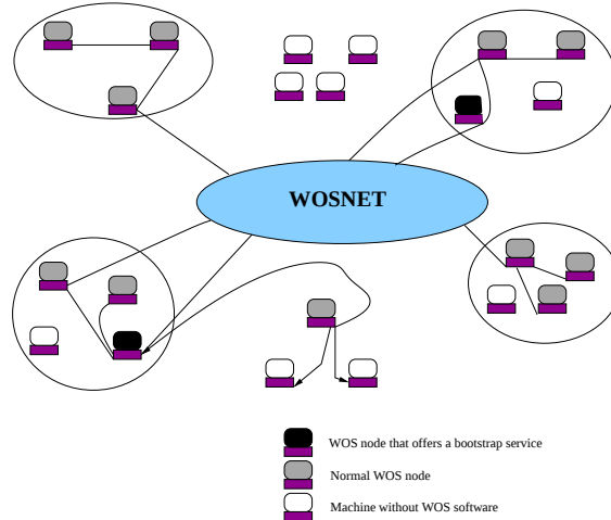
Figure 1: Bootstrap.
